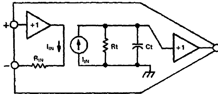
(b) Equivalent Schematic
