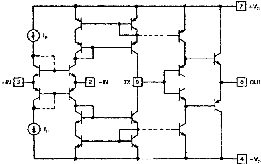
(a) Simplified Schematic
