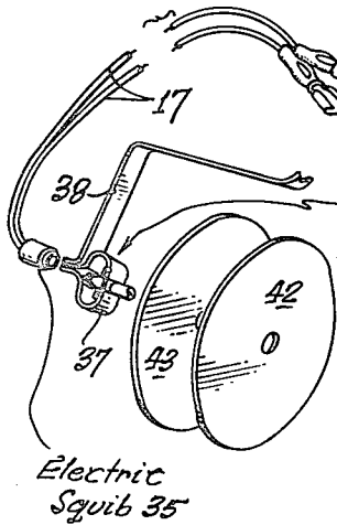
FIG. 4. Igniter Train 36
