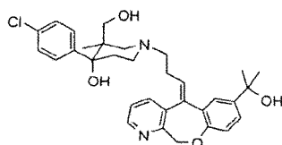
Example 483-1 (chiral) Example 483-2 (chiral)
