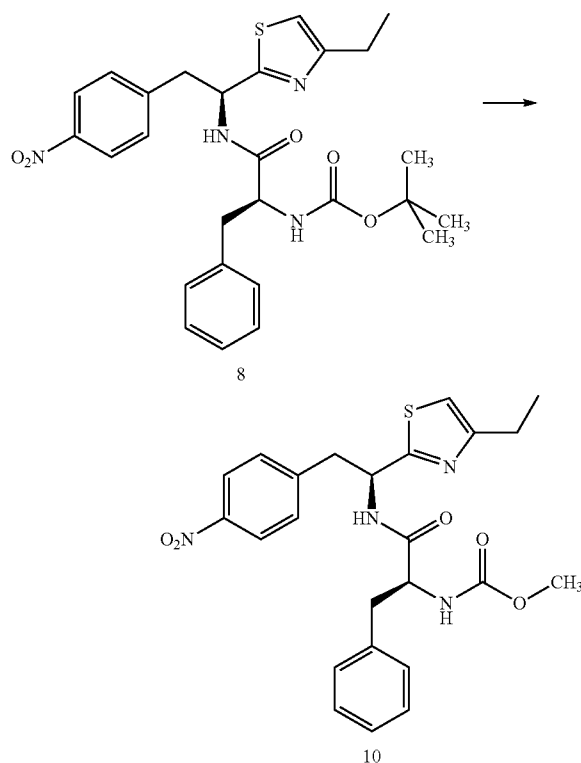
Scheme III
