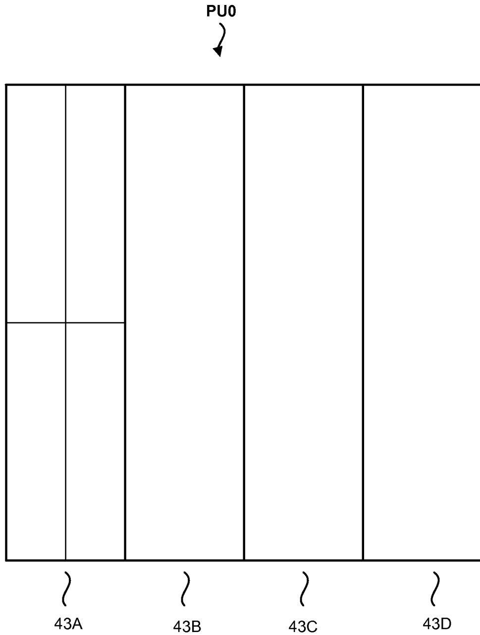
1/8Nx1/2N Partitioning of Sub-block 43A
