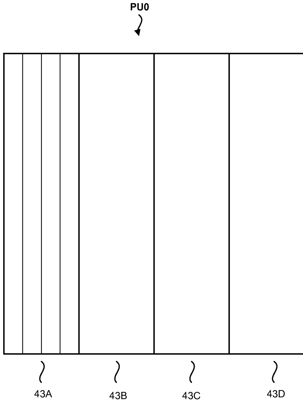
1/16NxN Partitioning of Sub-block 43A
