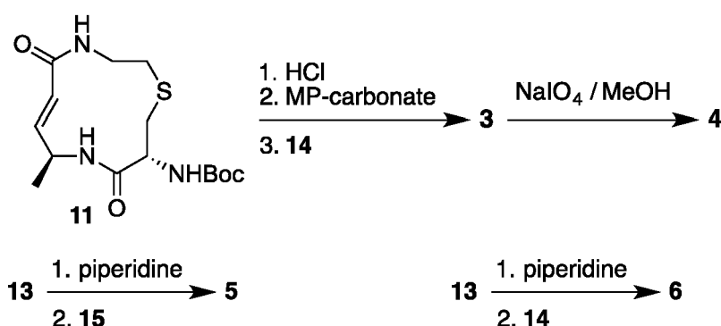
Scheme 3. Synthesis of thiasyrbactins 3-6
