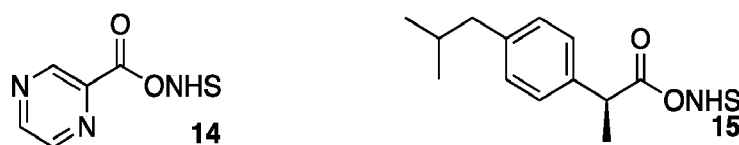
Chart 3. Side chain active esters.
