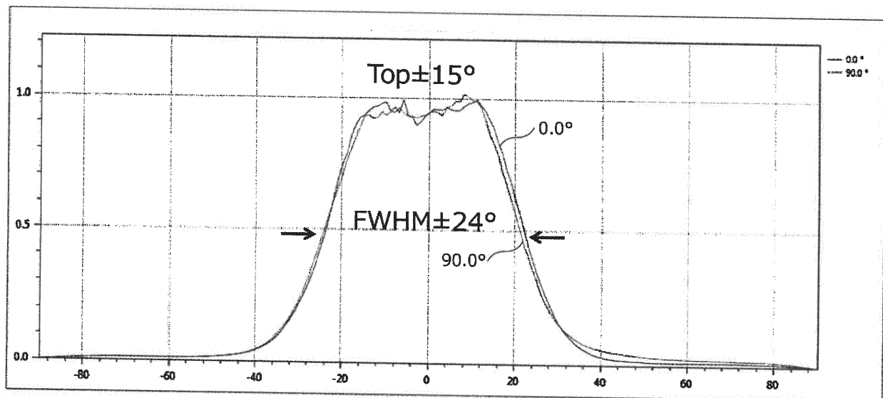
FIG. 18 BTDF (TRANSMISSION SCATTERING) \pm 35^\circ SYSTEM (CORRESPONDING TO \pm 20^\circ ) Resist-Master
