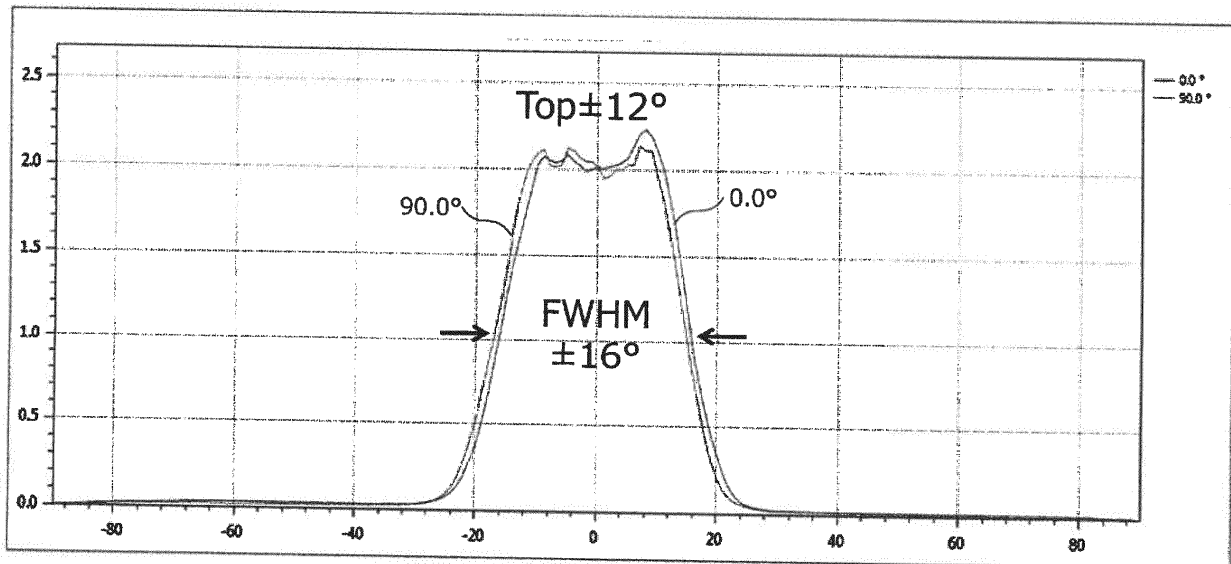
FIG. 16 BTDF (TRANSMISSION SCATTERING) \pm 18^\circ SYSTEM (CORRESPONDING TO \pm 13^\circ ) Resist Master
