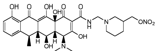
amido-N-[4-(nitrooxymethyl)piperidinomethyl]-α-6-deoxy-5-oxytetracycline
