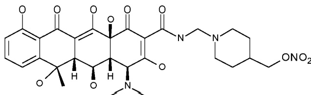
amido-N-[3-(nitrooxymethyl)piperidinomethyl]-tetracycline;
