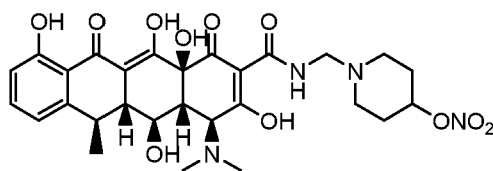
amido-N-[4-nitrooxypiperidinomethyl]-tetracycline
