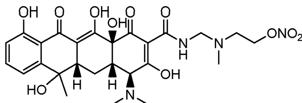
amido-N-[4-(nitrooxymethyl)piperidinomethyl]-tetracycline
