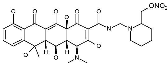
amido-N-[3-(nitrooxymethyl)piperidinomethyl]-tetracycline;
