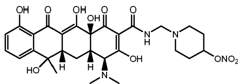
amido-N-[bis-(β-nitrooxyethyl)methylaminomethyl]-α-6-deoxy-5-oxytetracycline
