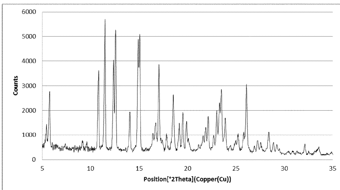
Figure 11. XRPD of (1R,2S)-(E)-2-(3-(4-((cis-2,6-dimethylmorpholino)methyl)styryl)-1H-indazol-6-yl)-5'-methoxySpiro[cyclopropane-1,3'-indolin]-2'-one maleate form A
