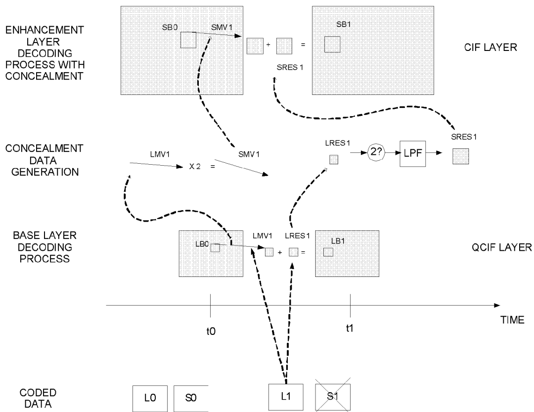
FIG. 8: CONCEALMENT PROCESS
