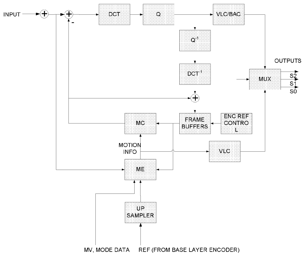
FIG. 6: SPATIAL SCALABILITY ENHANCEMENT LAYER CODEC
