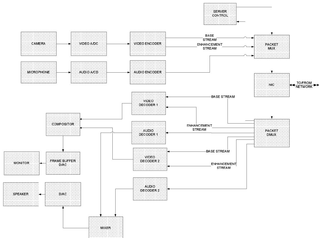
FIG. 2: END-USER TERMINAL
