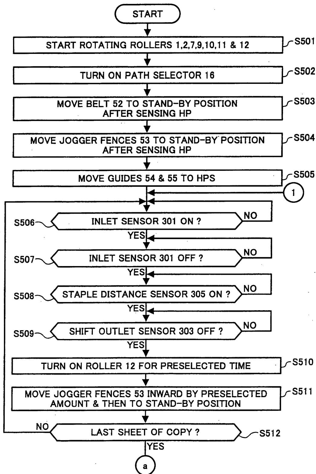
FIG. 22A CENTER STAPLE & FOLD MODE
