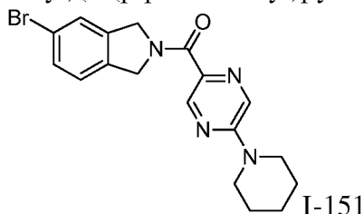
Intermediate 151 (5-Bromoisindolin-2-yl)(5-(piperidin-1-yl)pyrazin-2-yl)methanone
