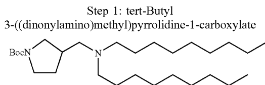
Chemical Formula: \text{C}_{28}\text{H}_{56}\text{N}_2\text{O}_2 Molecular Weight: 452.77
