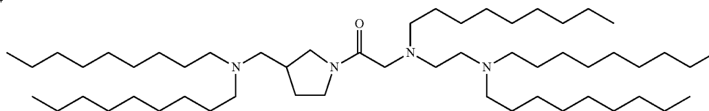
Chemical Formula: \text{C}_{54}\text{H}_{110}\text{N}_4\text{O} Molecular Weight: 831.50
