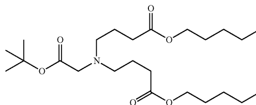
Chemical Formula: \text{C}_{24}\text{H}_{45}\text{NO}_6 Molecular Weight: 443.63
