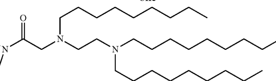
Chemical Formula: \text{C}_{54}\text{H}_{110}\text{N}_4\text{O} Molecular Weight: 831.50
