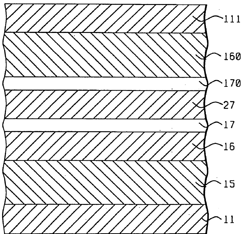
FIG. 3d
