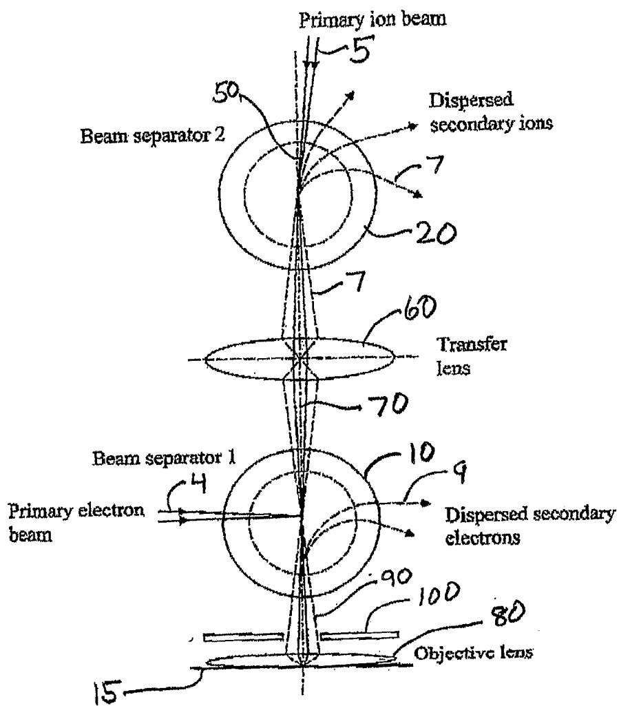
Figure 1: Schematic for ray paths of primary and scattered charged particles
