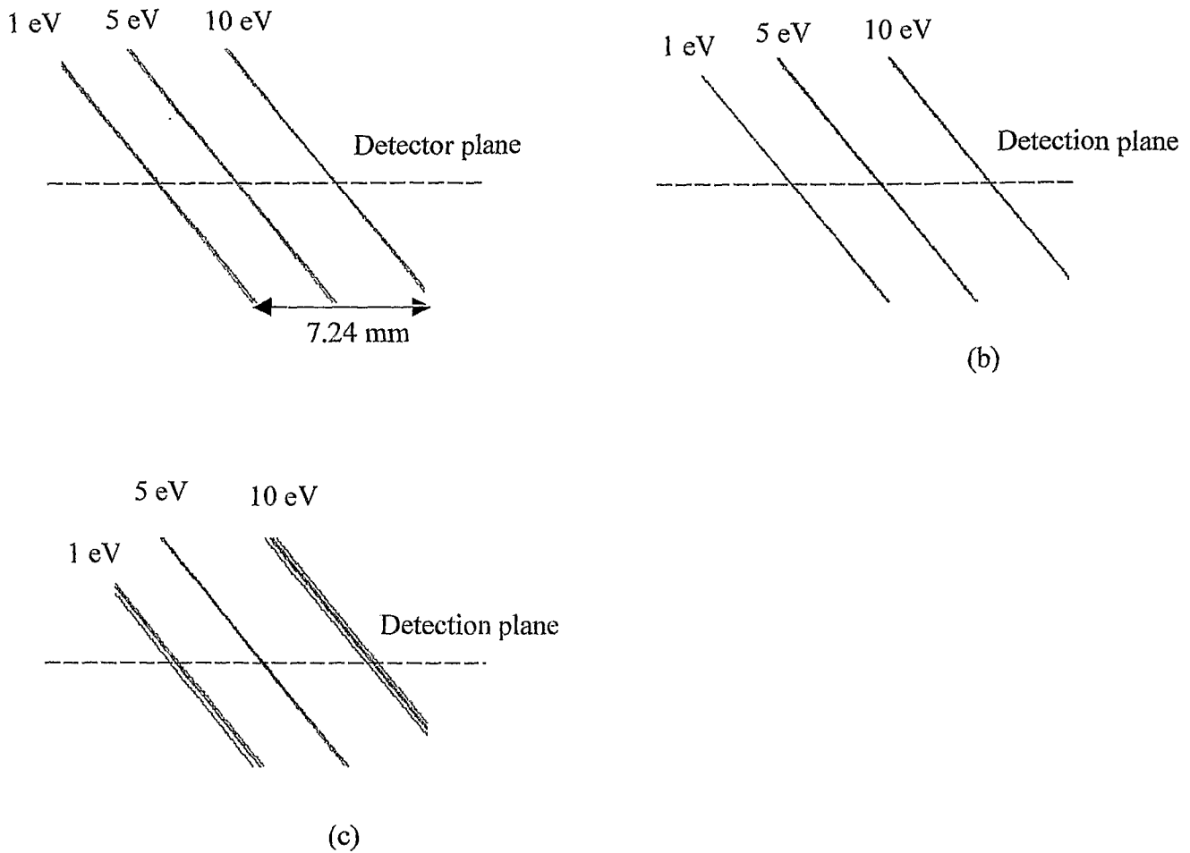
Figure 9: Simulated trajectory paths as they arrive at the detection plane for secondary gold ions emitted with energies of 1, 5, and 10 eV from a -1 kV biased specimen
