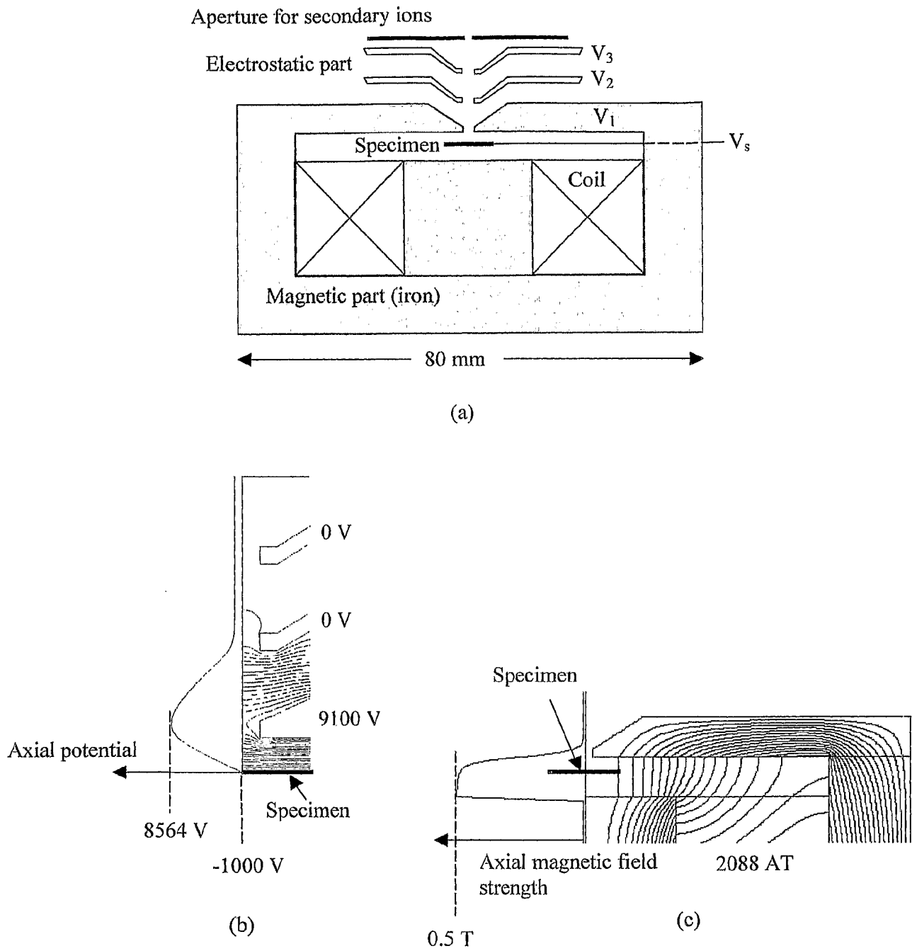
Figure 6: Simulated objective lens design
