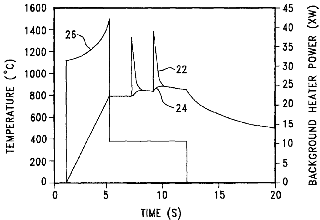
FIG. 3 (PRIOR ART)
