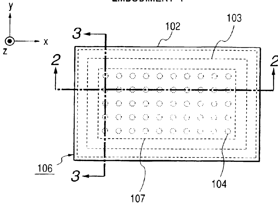
FRONT VIEW OF VACUUM CHAMBER EMBODIMENT 1
