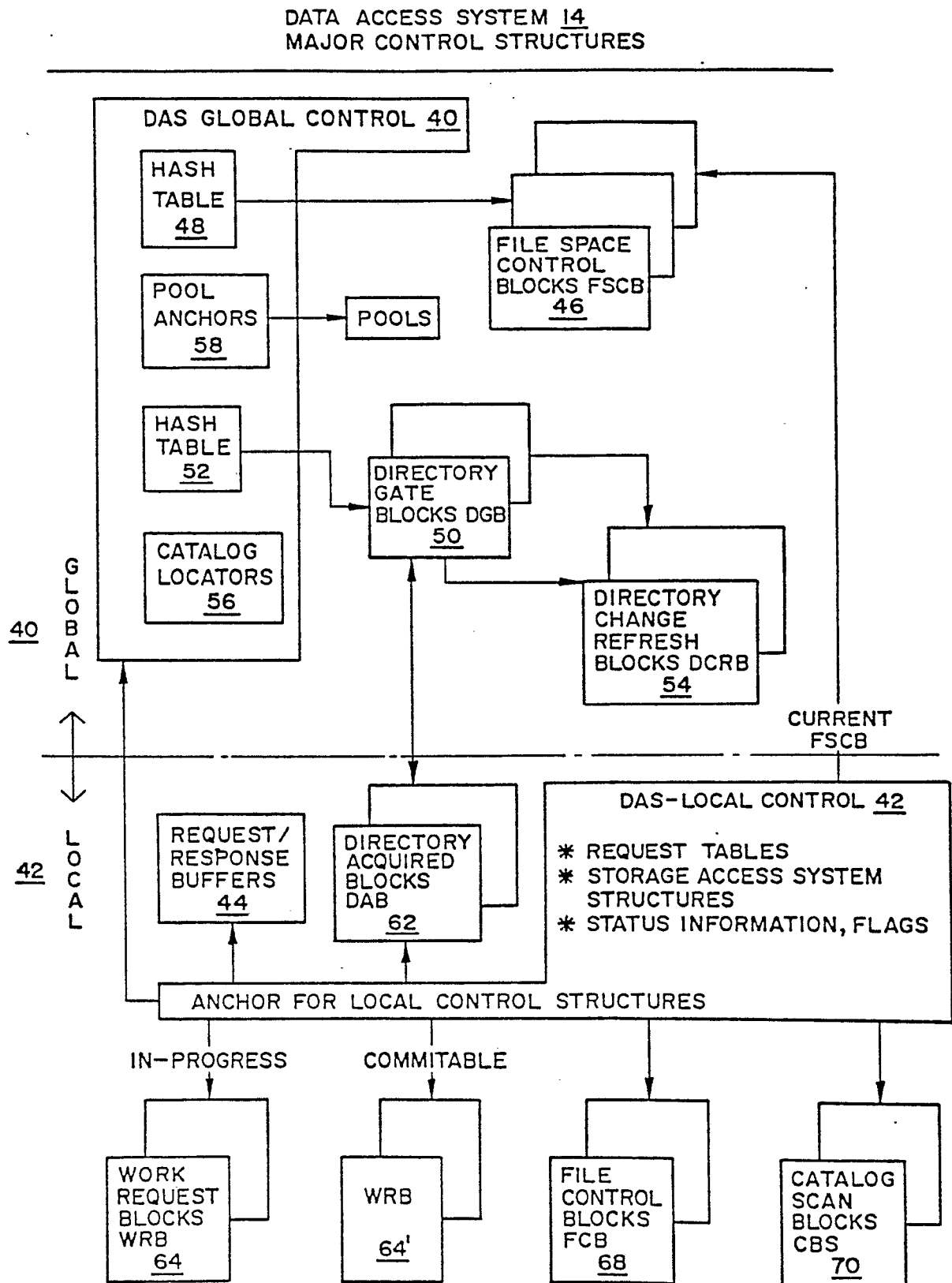
FIG.2 MAJOR DATA ACCESS SYSTEM CONTROL STRUCTURES
