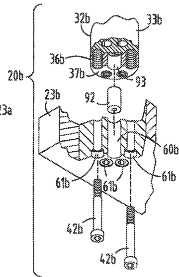
FIG. 22 PRIOR ART
