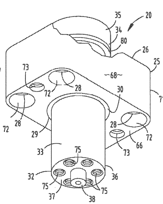
FIG. 3 PRIOR ART
