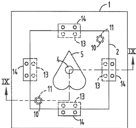
FIG. 8 PRIOR ART
