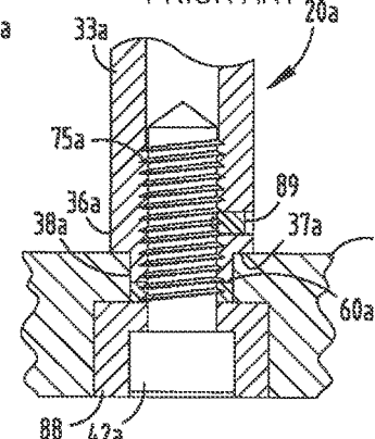
FIG. 20 PRIOR ART
