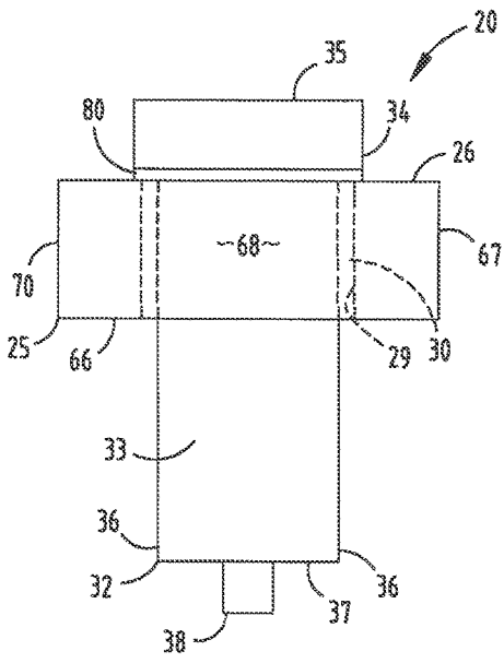
FIG. 2 PRIOR ART
