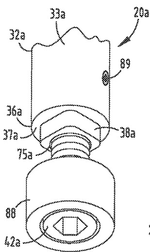
FIG. 19 PRIOR ART
