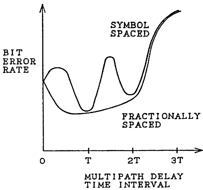
FIG. 23 (PRIOR ART)
