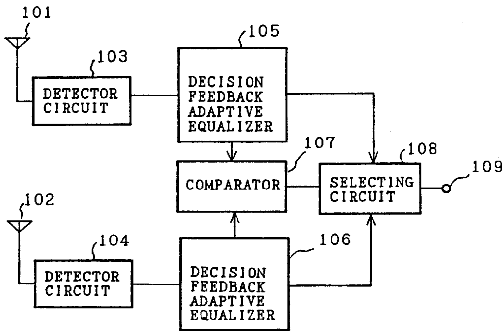
FIG. 21 (PRIOR ART)
