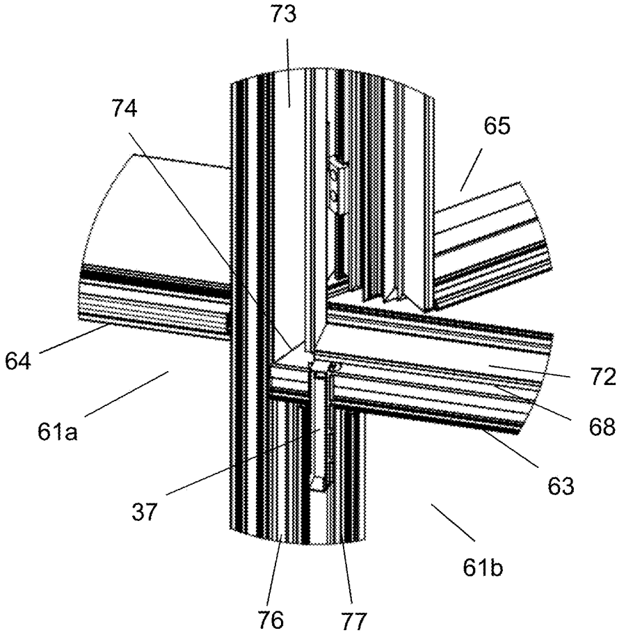
Detail C
