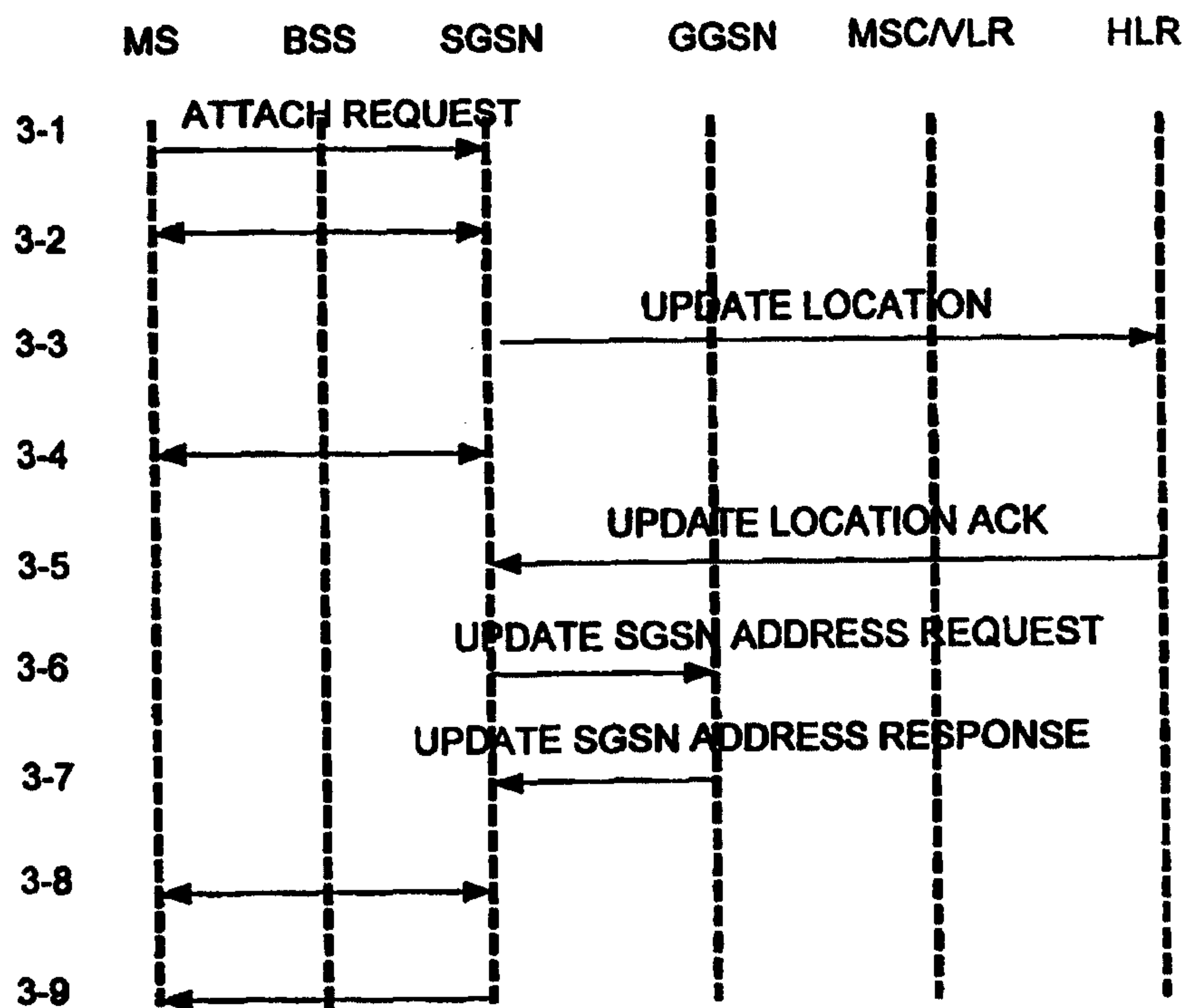
COMBINED IMSI/GPRS ATTACH PROCEDURE
