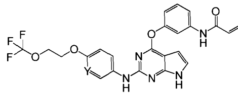
I-33 (Y = CH, CF, N)
