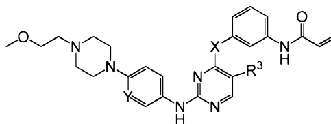
I-41 (X=O, NH, CH 2 , CF 2 ; Y=CH, CF, N; R 3 =OCH 3 , F)
