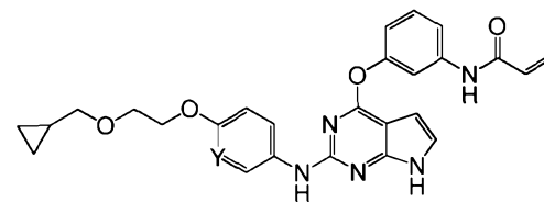
I-35 (Y = CH, CF, N)
