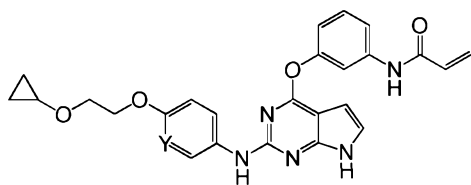
I-40 (Y = CH, CF, N)
