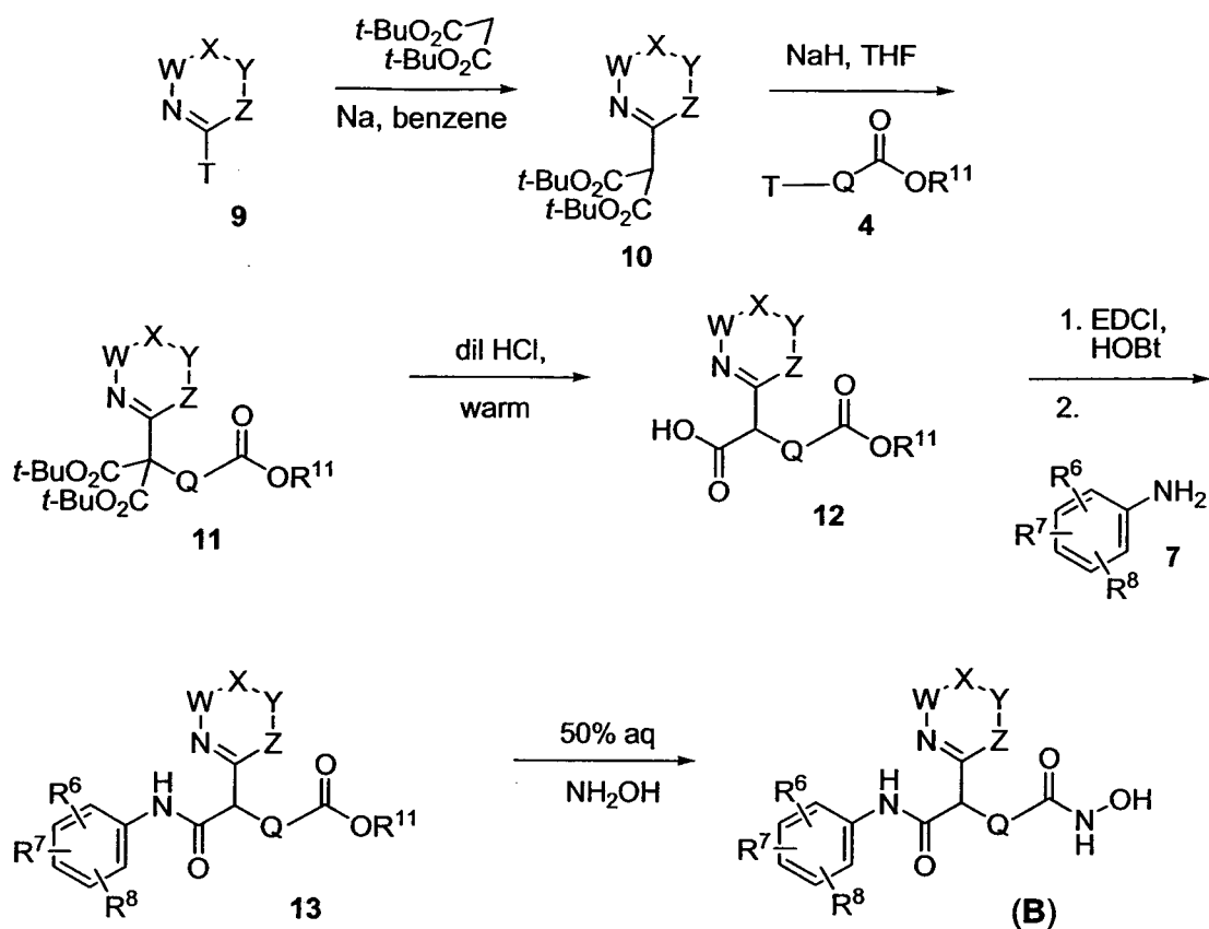
Scheme 3
