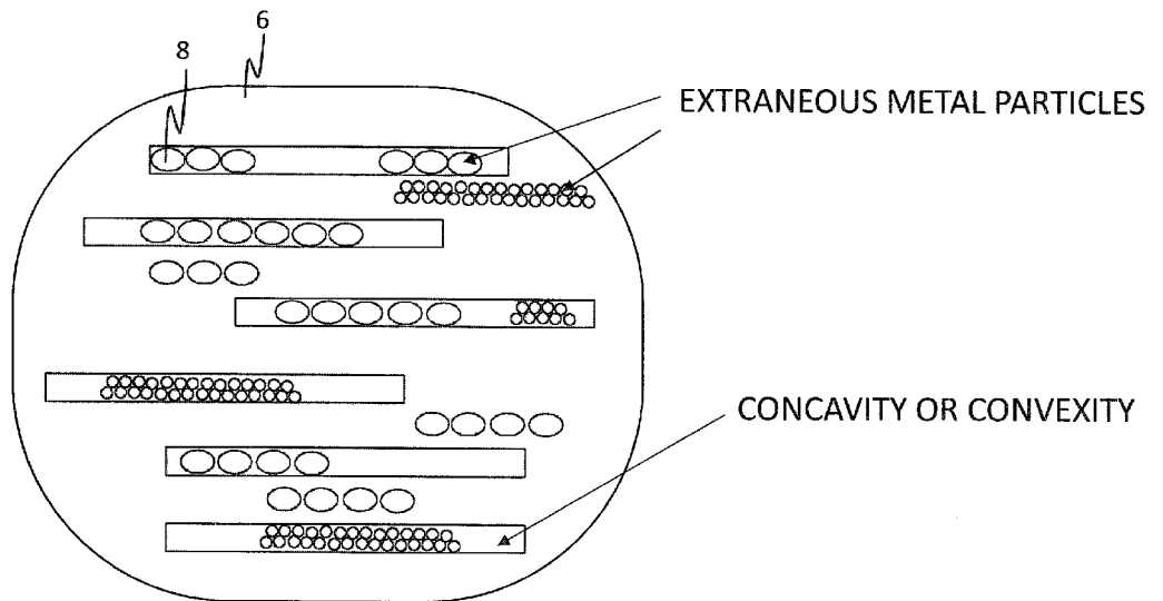
DIAGRAM VIEWED FROM ABOVE (FLAT SURFACE OF FLAKY MAGNETIC METAL PARTICLE)
