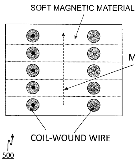
EXEMPLARY CONCEPTUAL CROSS-SECTIONAL VIEW OF CHIP INDUCTOR
