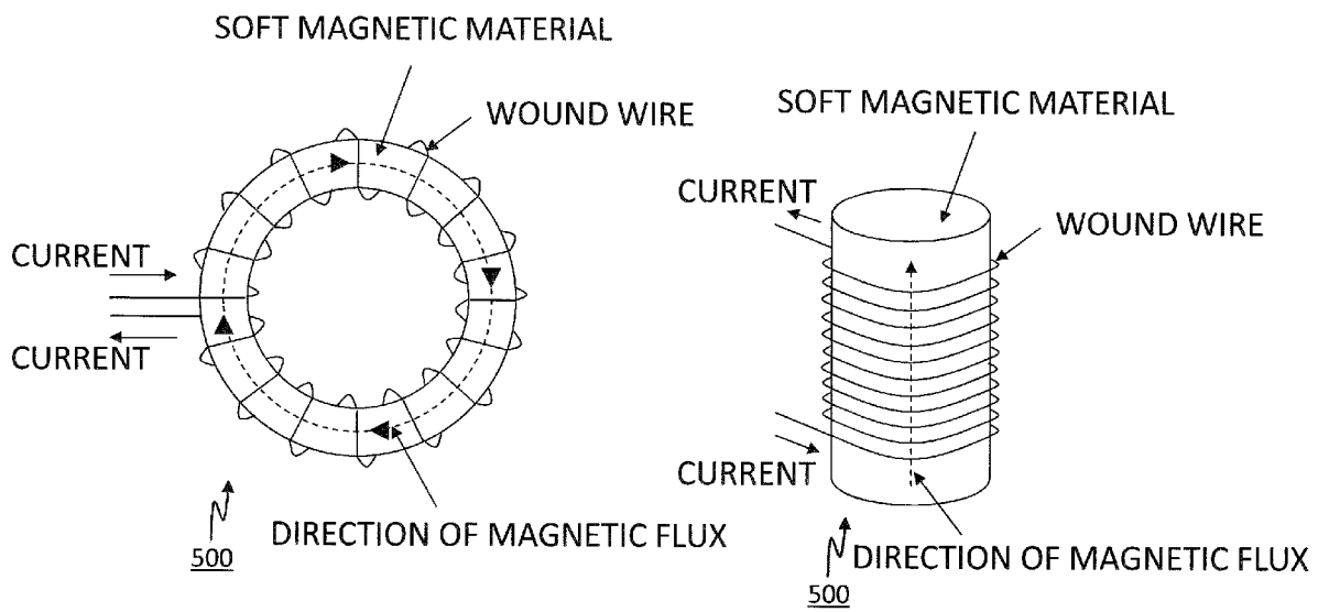
EXEMPLARY CONCEPTUAL DIAGRAM OF RING-SHAPED INDUCTOR
