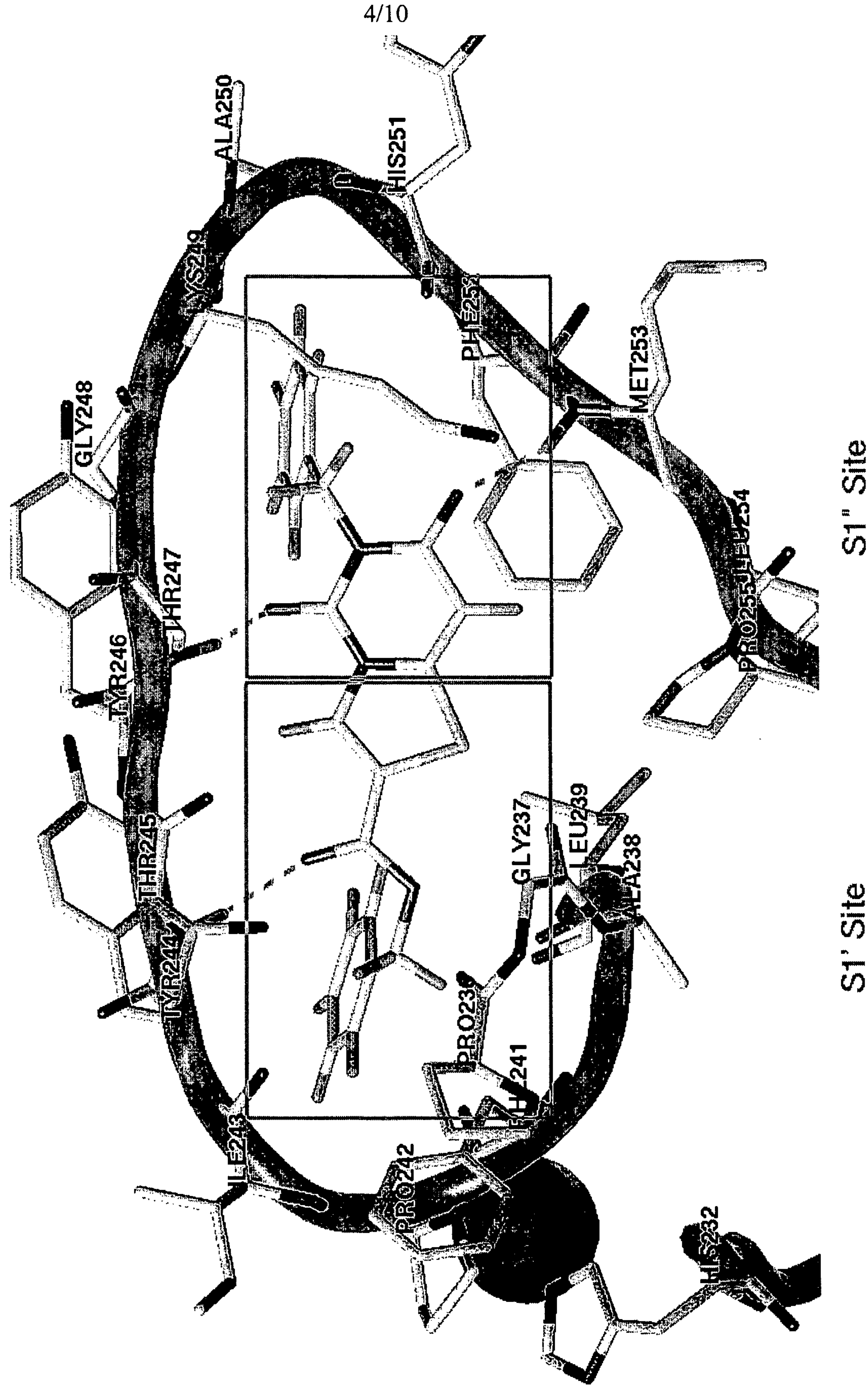
Figure 3: Synthesis example 1 binding mode
