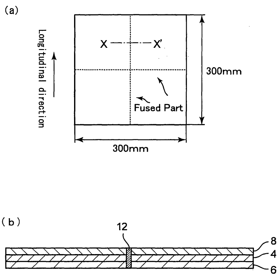
Cross section of Joint (X-X' cross section view)
