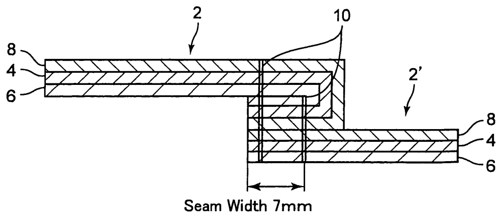
Cross section of Joint (X-X' cross section view)
