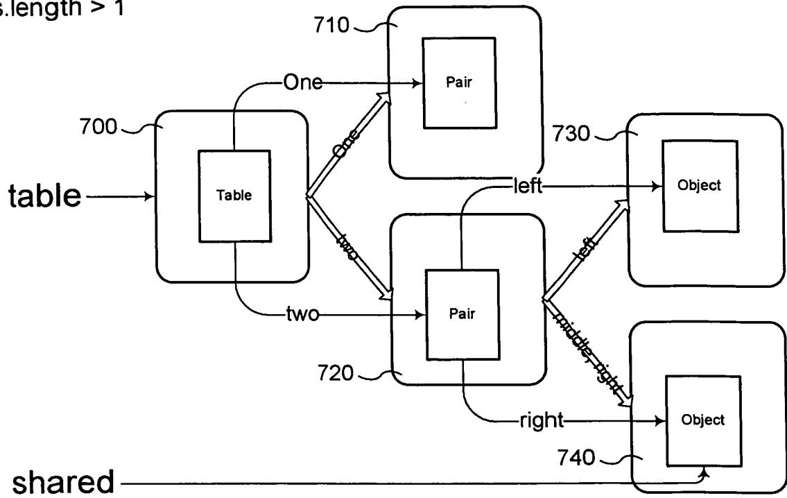
Fig. 7b args.length ≤ 1
