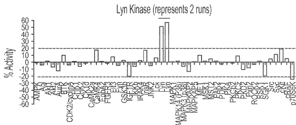
Compound 102 - Activation of Lyn Kinase in vitro
