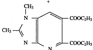
Isomer B
