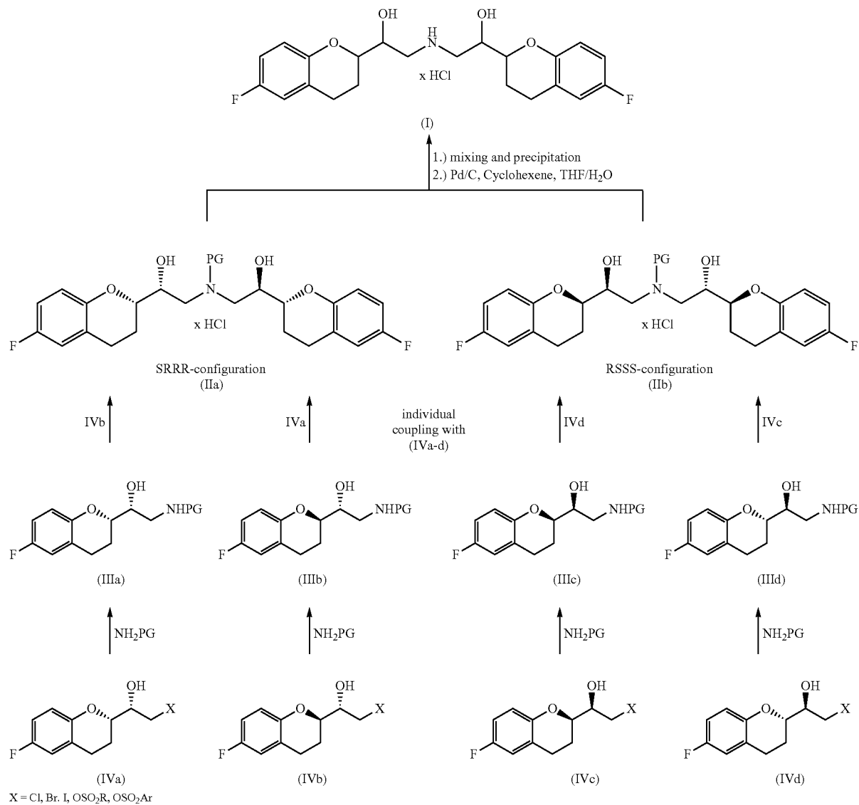
Scheme 2: Overall Synthesis
