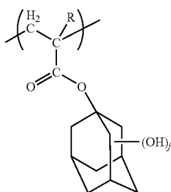
[Chemical Formula 31.]
