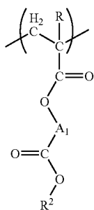
[Chemical Formula 48.]
