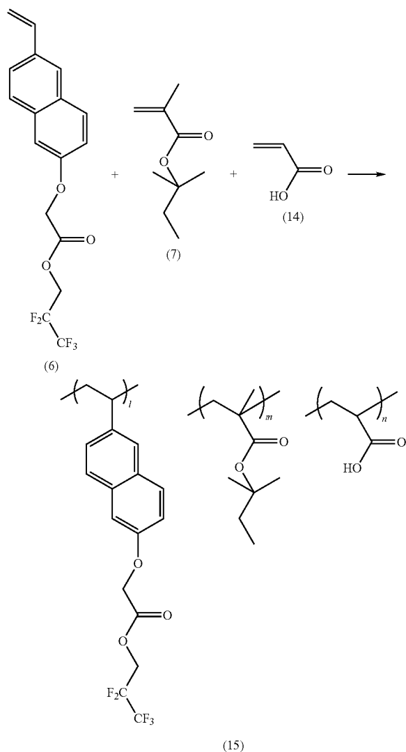
[Chemical Formula 84.]
