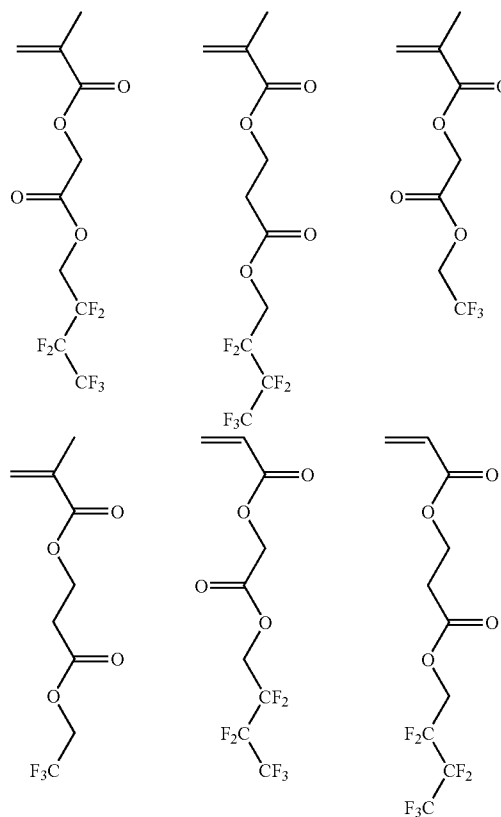
[Chemical Formula 45.]
