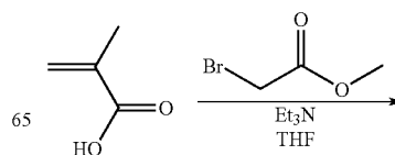
[Chemical Formula 85.]
