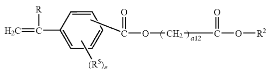
(c-1-19)
