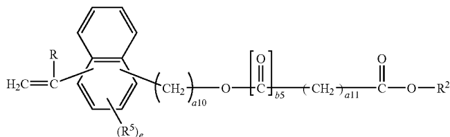
(c-1-19)
