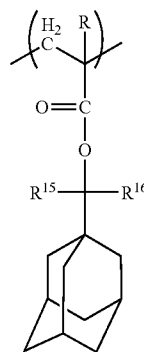
[Chemical Formula 3.]
