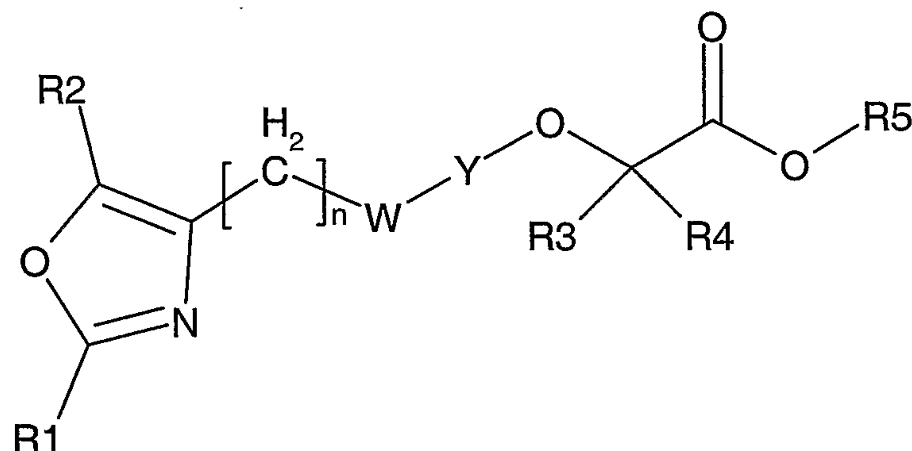
Structural Formula I
