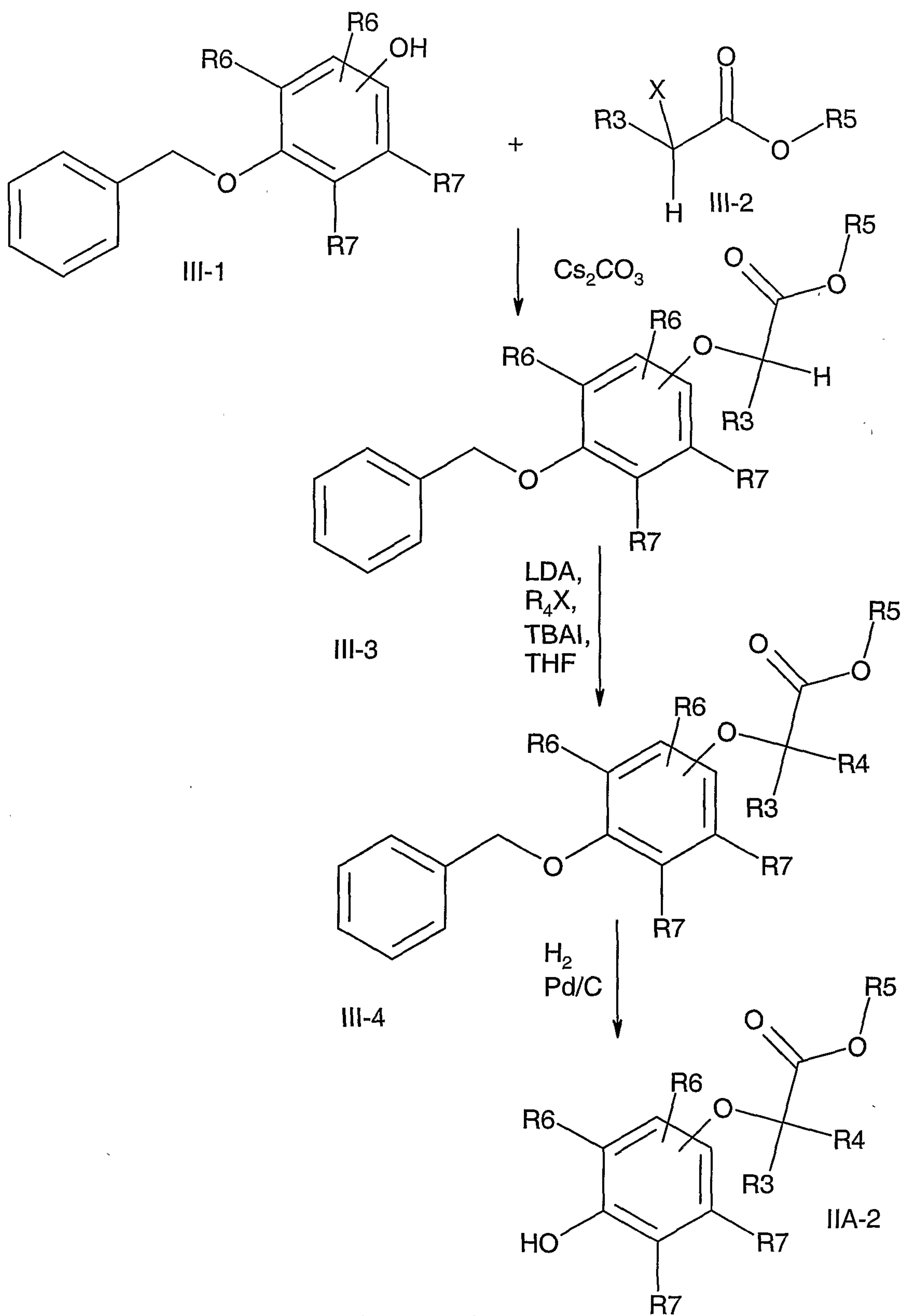
Scheme III
