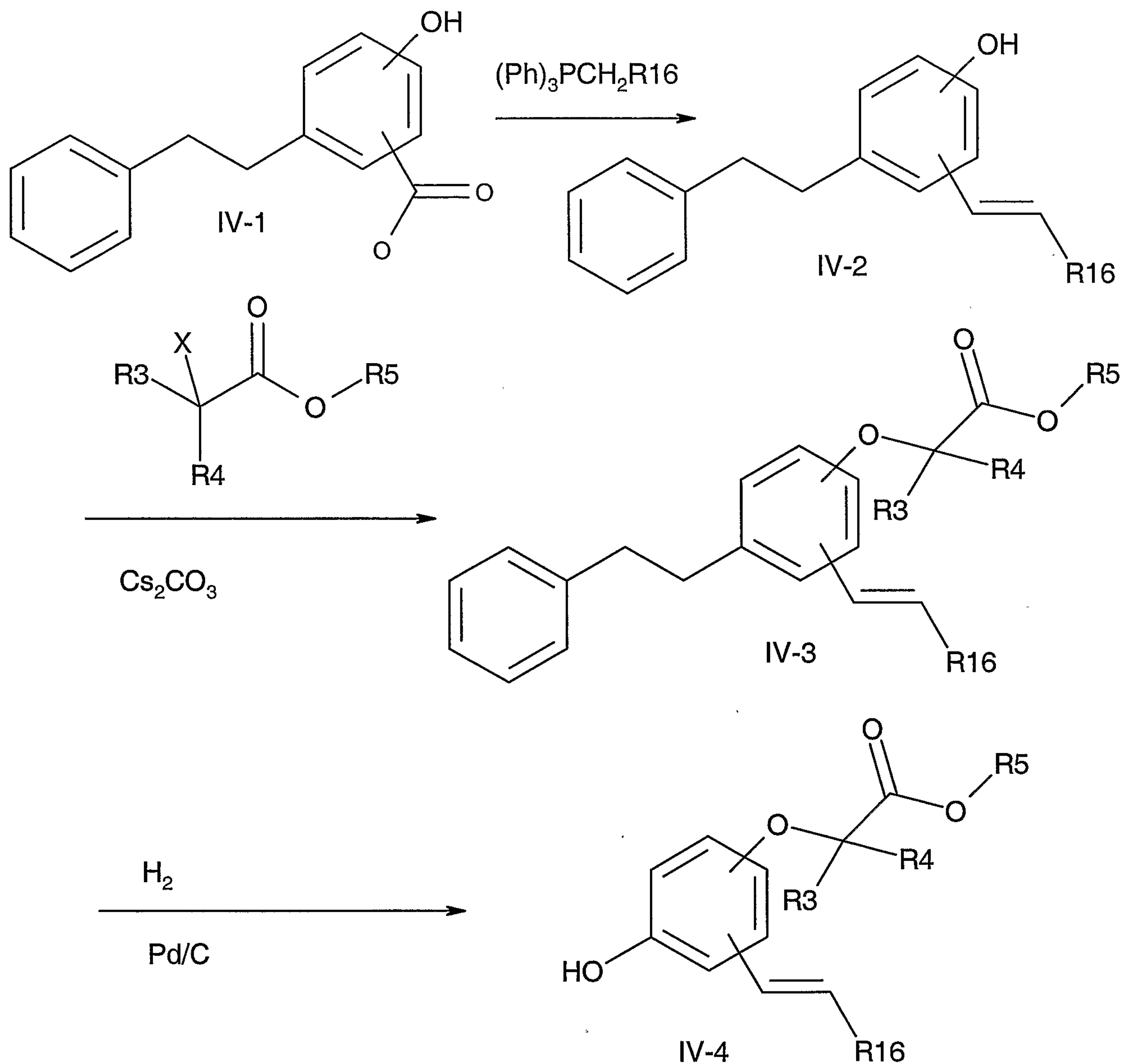
Scheme IV
