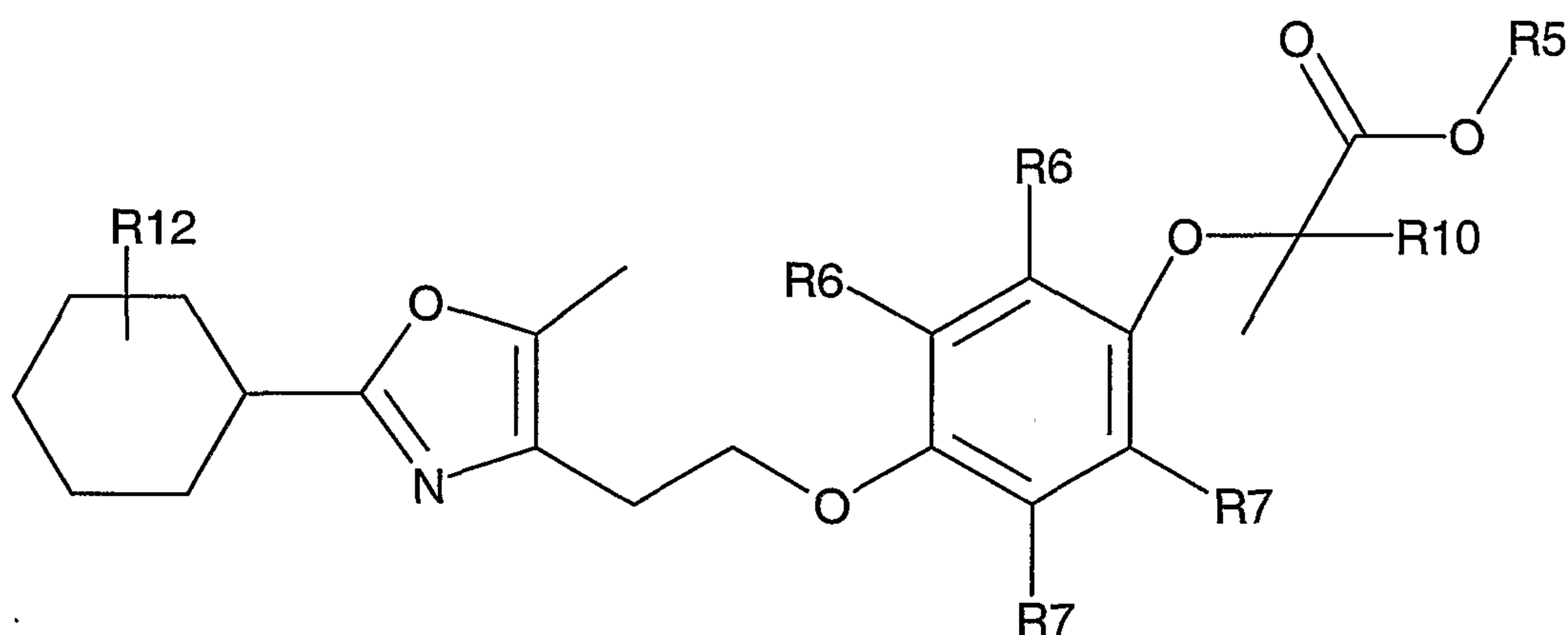
10 Structural Formula IV
