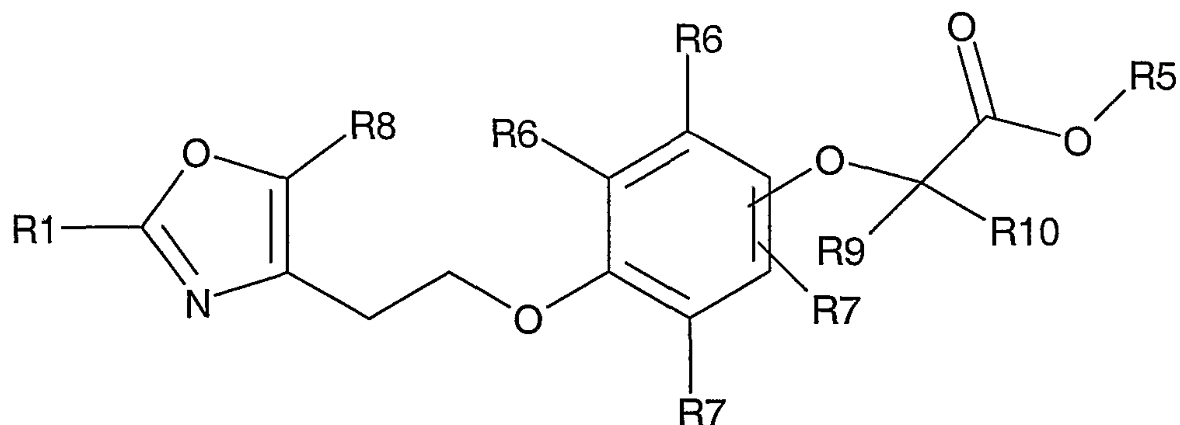
Structural Formula IIa:
