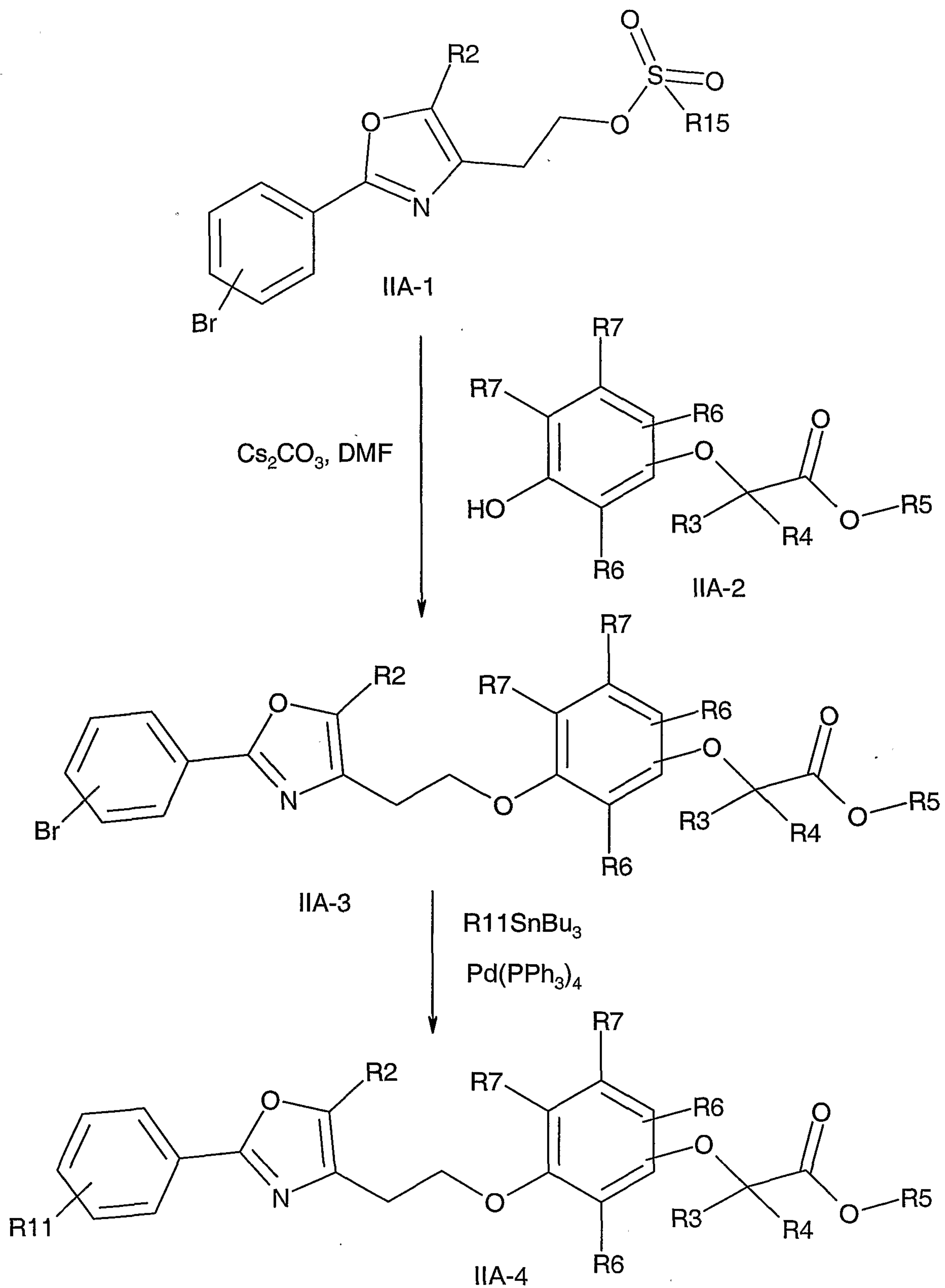
Scheme IIA
