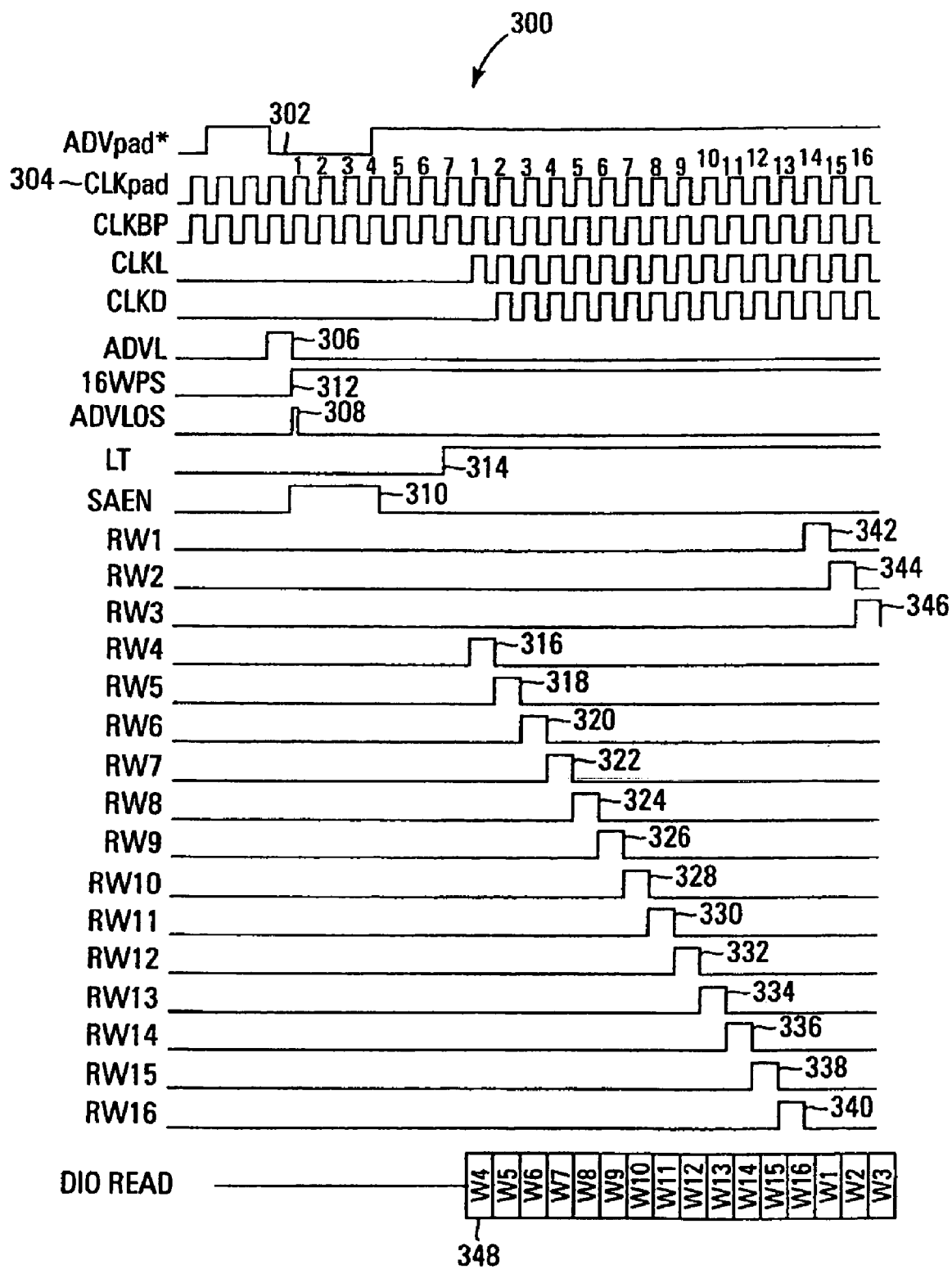
Fig. 3 Prior Art
