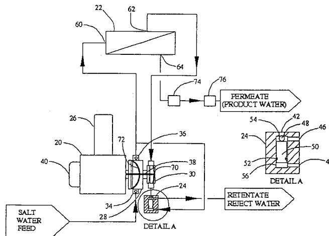
DUAL DIAPHRAGM PUMP DRIVEN MEMBRANE SYSTEM
