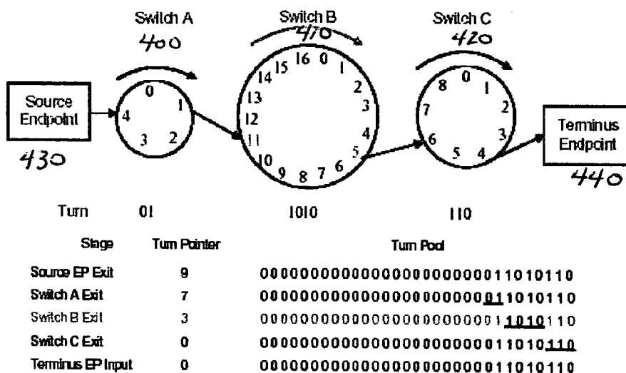
Figure 4. Example of forward routing using AS
