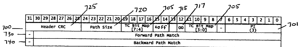
Figure 7: Transaction Layer Packet per present invention
