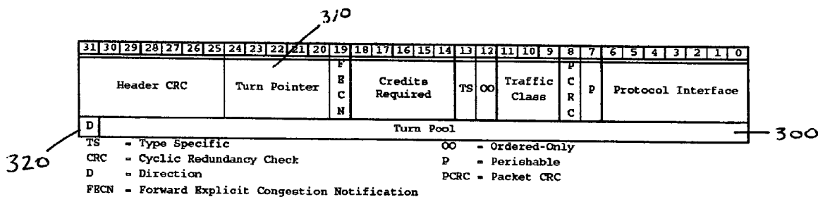
Packet header in accordance with AS specification
