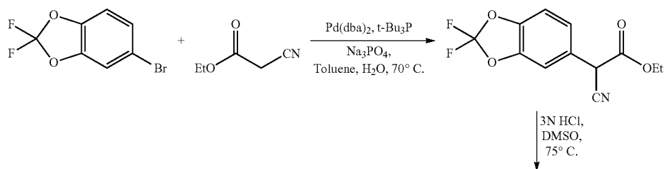
Scheme 2. Alternative synthesis of the acid chloride moiety.
