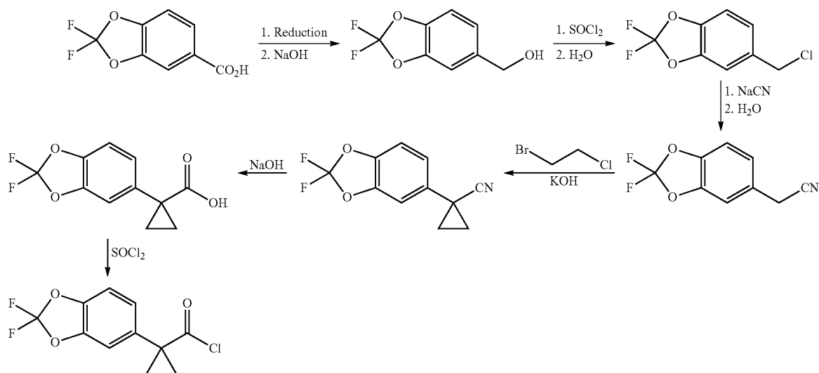
Scheme 1. Synthesis of the acid chloride moiety.
