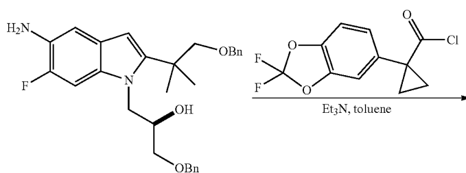
Scheme 4. Formation of Compound 1.
