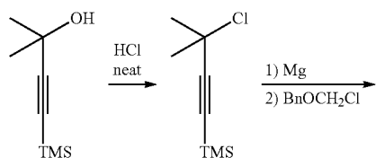
Scheme 3. Synthesis of the amine moiety.
