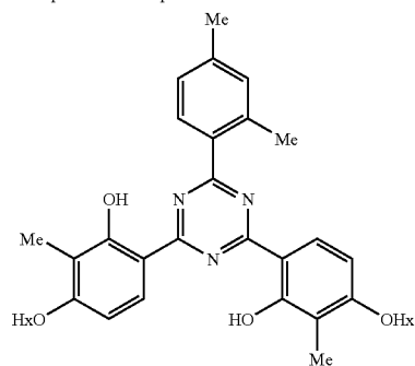
Comparative Compound 3
