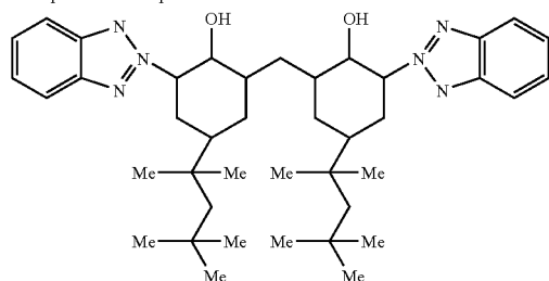
Comparative Compound 3
