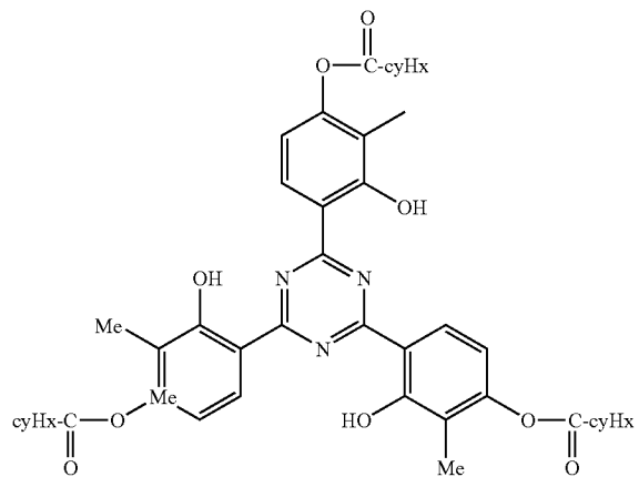
Compound 28
