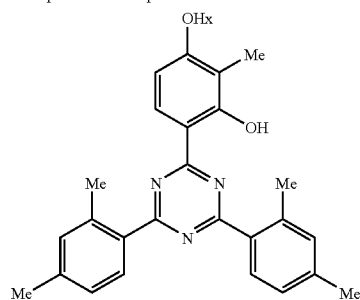
Comparative Compound 2
