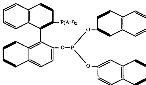
(R,S)-BINAPHOS
