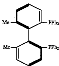
(S)-BICHEP
