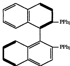
(R)-BINAP
