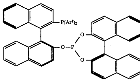
(S,R)-BINAPHOS
