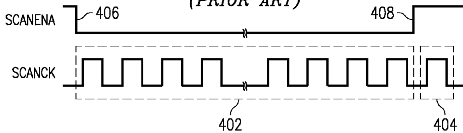
FIG. 4 (PRIOR ART)
