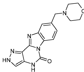
(XXXIIIa)
