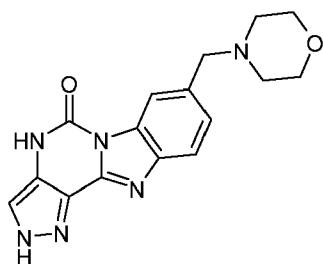
(XXXIII)
