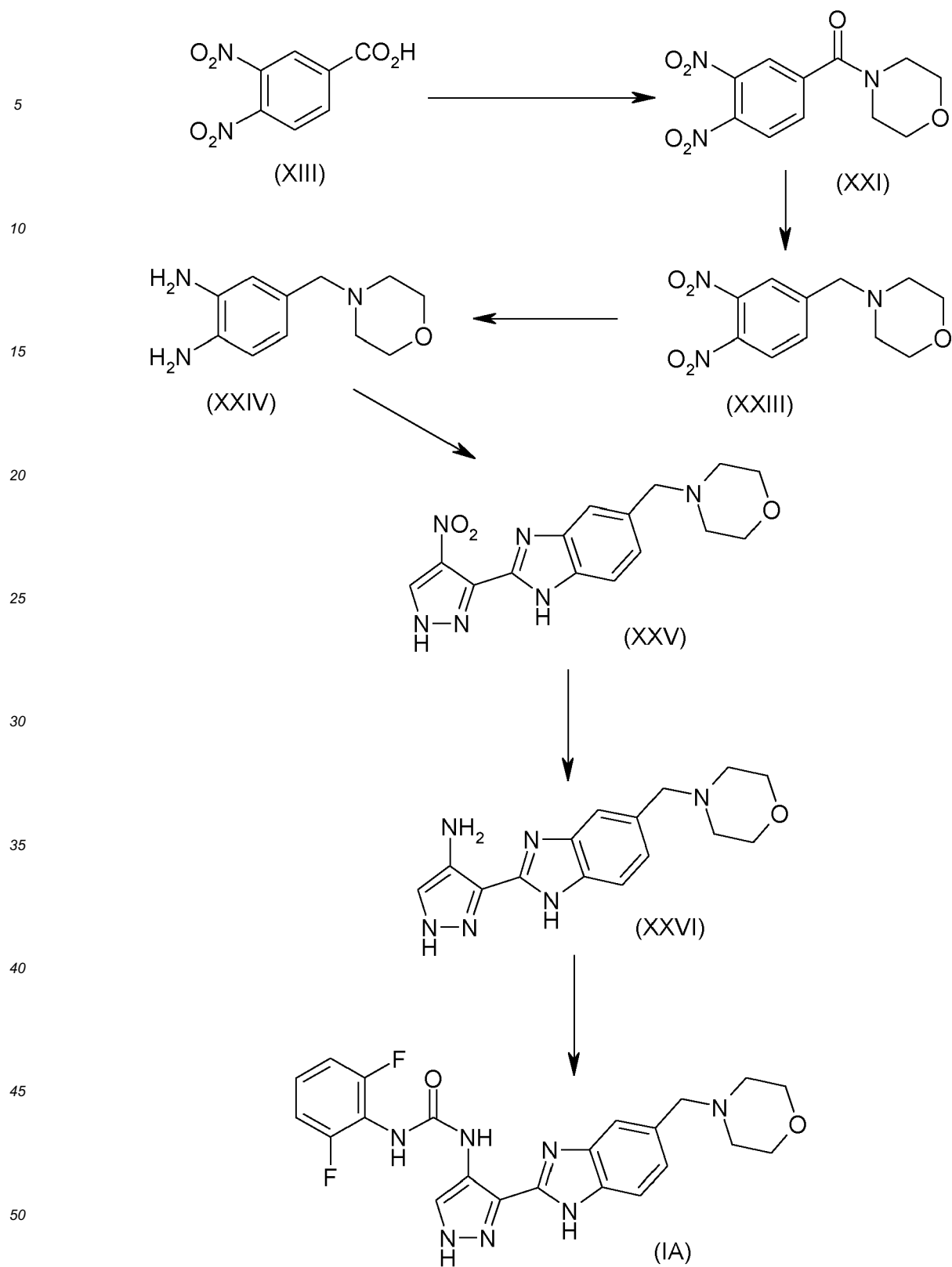
Scheme 3
