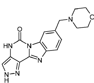
(XXXIII)
