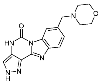
(XXXIII)
