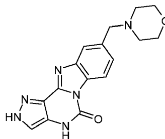
(XXXIIIa)
