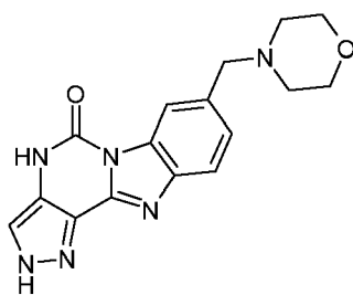
(XXXIII)
