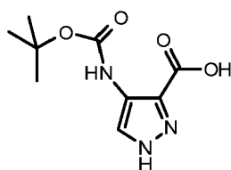
(XXXII)
