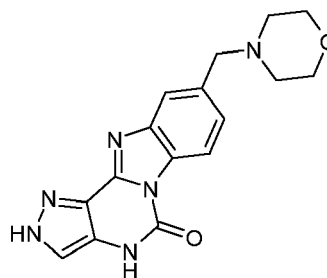
(XXXIIIa)
