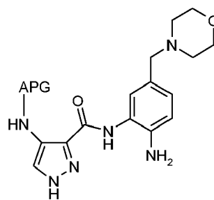
(XXVIIIa)
