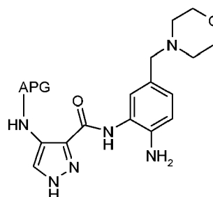
(XXVIIIa)
