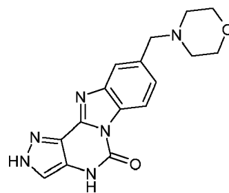
(XXXIIIa)
