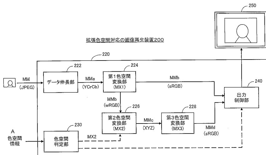
200. EXPANDED-COLOR-SPACE-CAPABLE IMAGE REPRODUCING APPARATUS 222.. DATA DECOMPRESSING PART 224.. FIRST COLOR SPACE CONVERTING PART (MX1) 240.. OUTPUT CONTROL PART A.. COLOR SPACE INFORMATION 230.. COLOR SPACE DETERMINING PART 226.. SECOND COLOR SPACE CONVERTING PART (MX2) 228.. THIRD COLOR SPACE CONVERTING PART (MX3)
