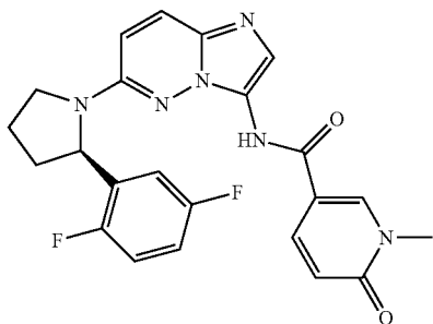
(R)—N-(6-(2-(2,5-difluorophenyl)pyrrolidin-1-yl)imidazo[1,2-b]pyridazin-3-yl)-1-methyl-6-oxo-1,6-dihydropyridine-3-carboxamide
