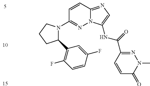
(R)—N-(6-(2-(2,5-difluorophenyl)pyrrolidin-1-yl)imidazo[1,2-b]pyridazin-3-yl)-1-methyl-6-oxo-1,6-dihydropyridazine-3-carboxamide
