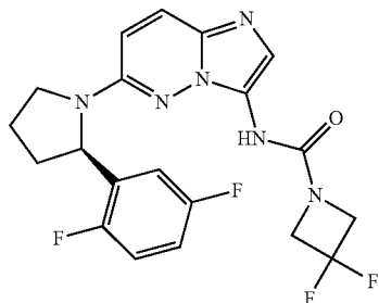
(R)-N-(6-(2-(2,5-difluorophenyl)pyrrolidin-1-yl)imidazo[1,2-b]pyridazin-3-yl)-3,3-difluoroazetidine-1-carboxamide
