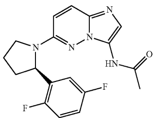
(R)—N-(6-(2-(2,5-difluorophenyl)pyrrolidin-1-yl)imidazo[1,2-b]pyridazin-3-yl)acetamide
