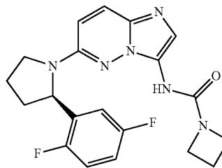
(R)-N-(6-(2-(2,5-difluorophenyl)pyrrolidin-1-yl)imidazo[1,2-b]pyridazin-3-yl)azetidine-1-carboxamide
