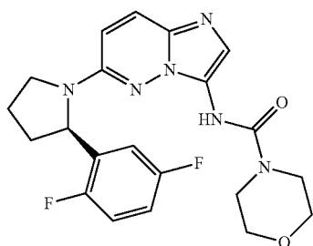
(R)—N-(6-(2-(2,5-difluorophenyl)pyrrolidin-1-yl)imidazo[1,2-b]pyridazin-3-yl)morpholine-4-carboxamide
