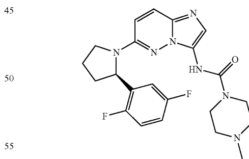
(R)—N-(6-(2-(2,5-difluorophenyl)pyrrolidin-1-yl)imidazo[1,2-b]pyridazin-3-yl)-4-methylpiperazine-1-carboxamide
