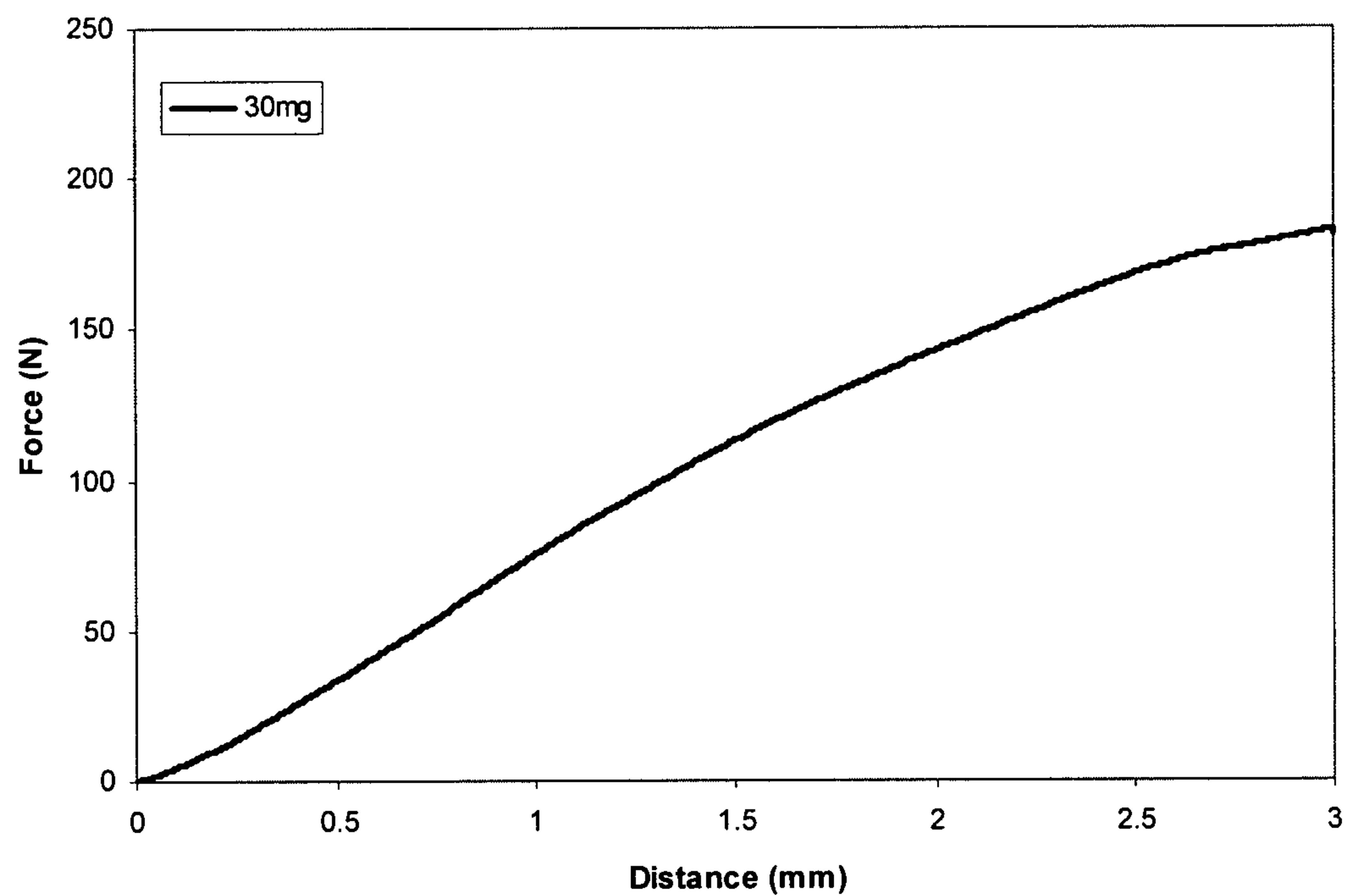
Example 20 Indentation Test of Example 13.4 tablet
