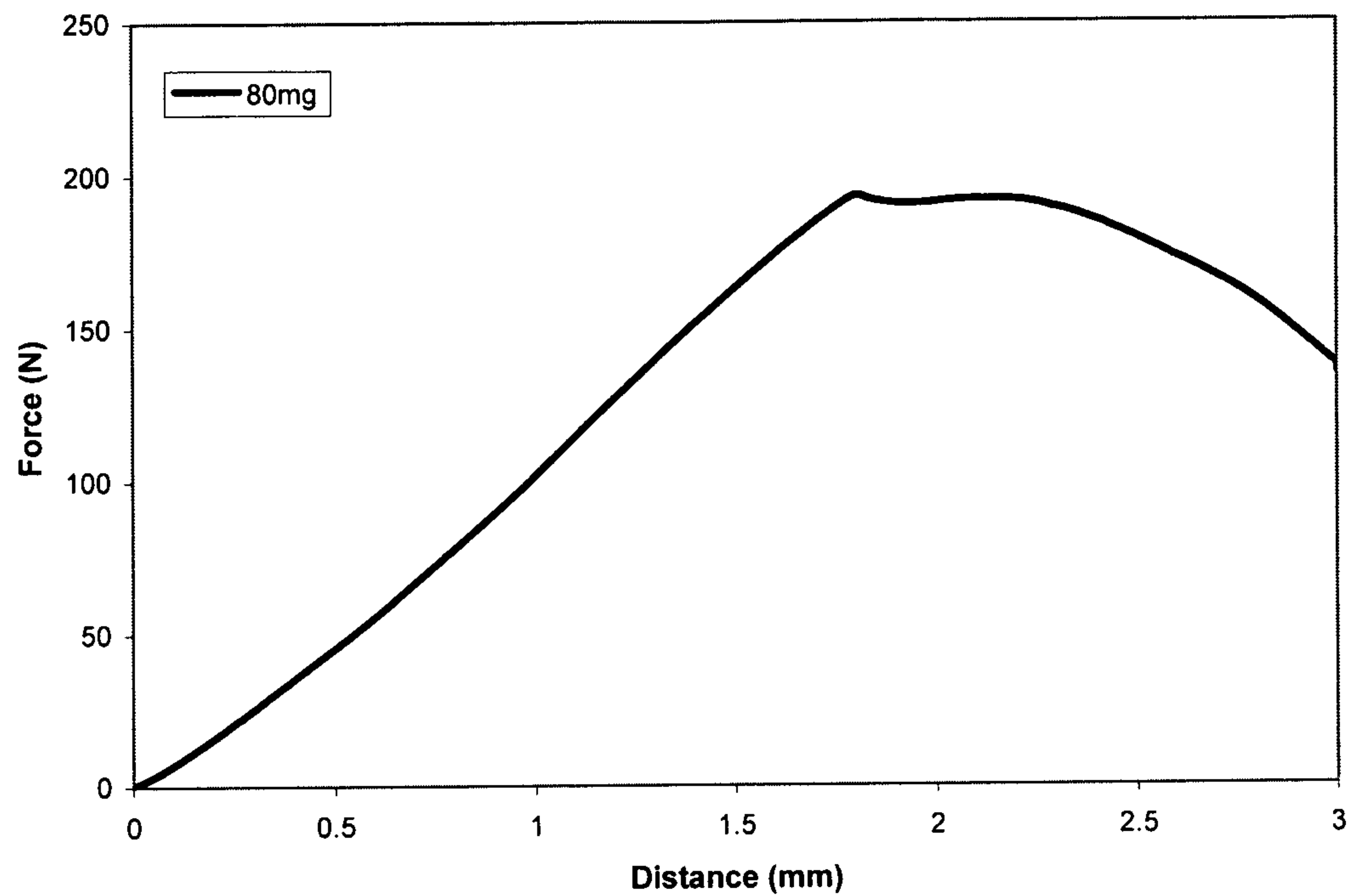
Example 20 Indentation Test of Example 18.2 tablet
