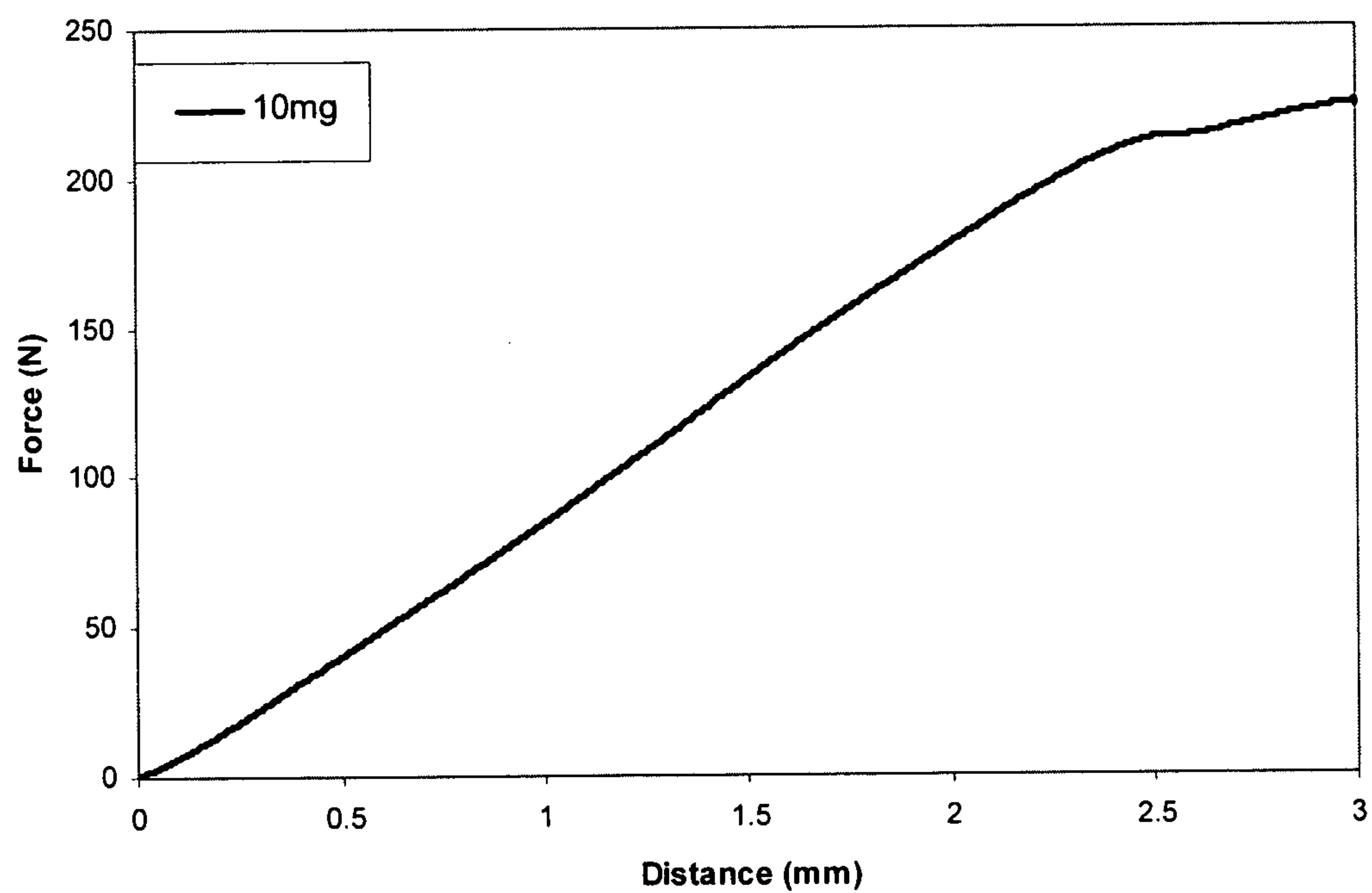
Example 20 Indentation Test of Example 14.1 tablet
