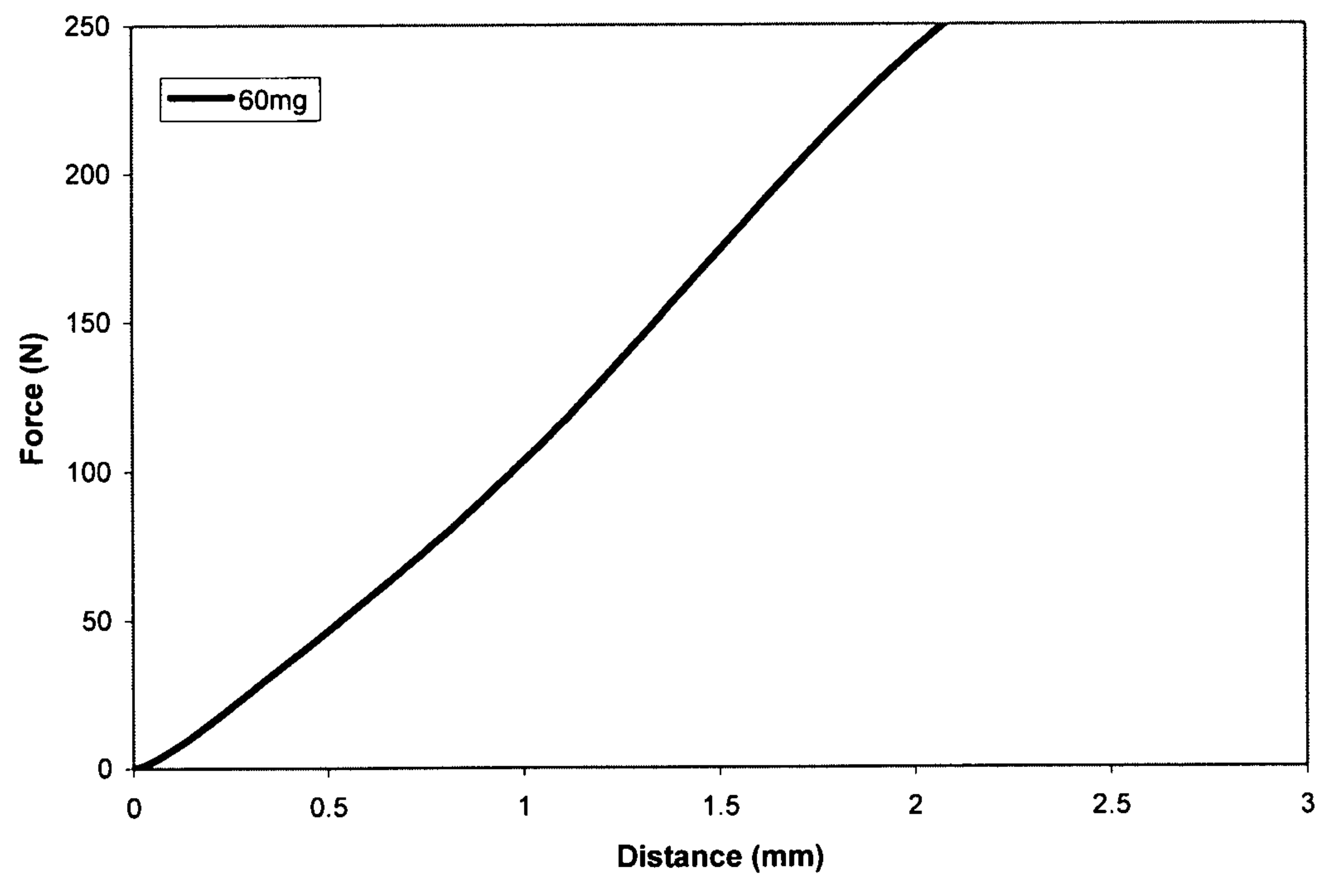
Example 20 Indentation Test of Example 17.1 tablet
