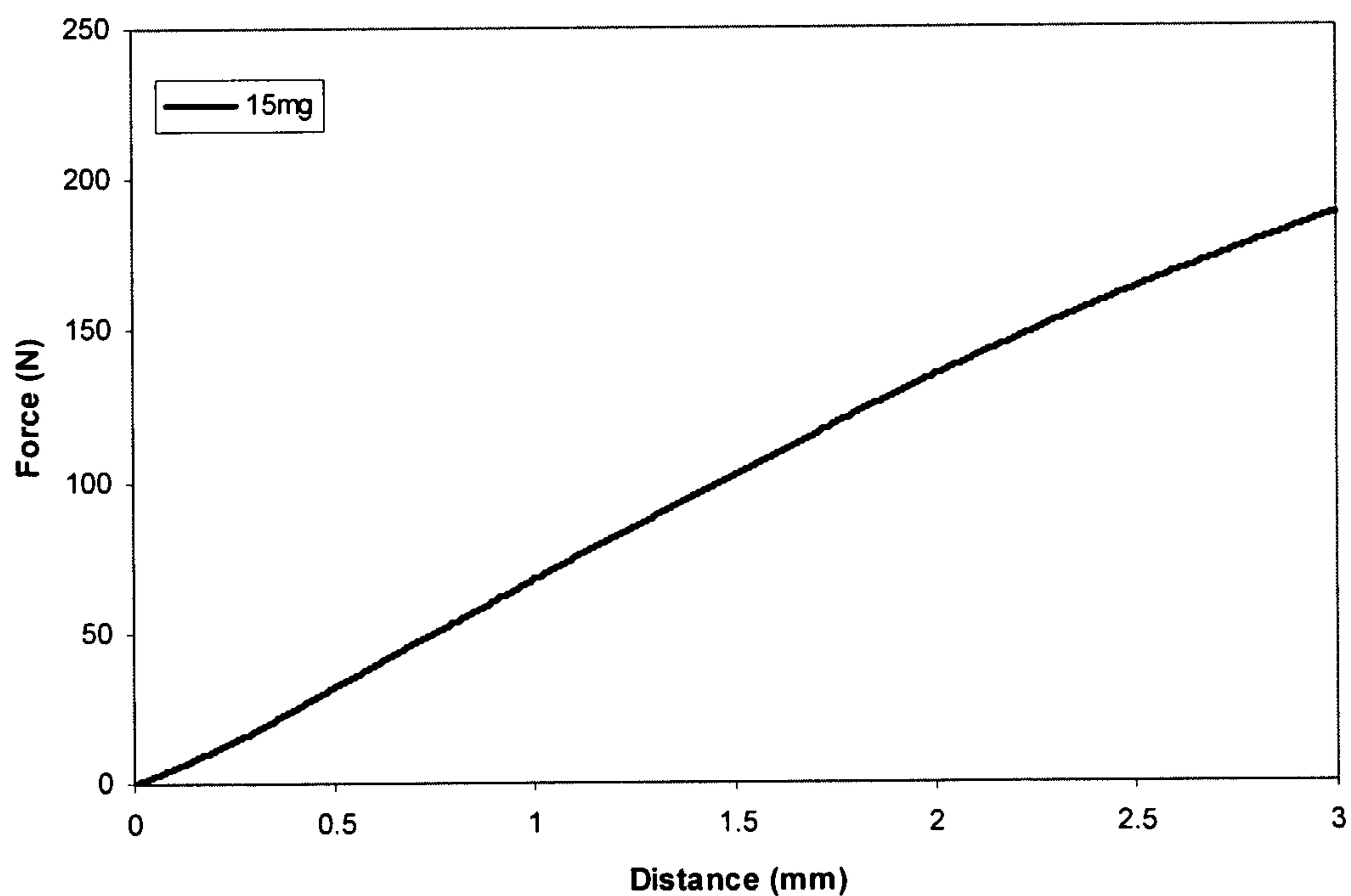
Example 20 Indentation Test of Example 13.2 tablet
