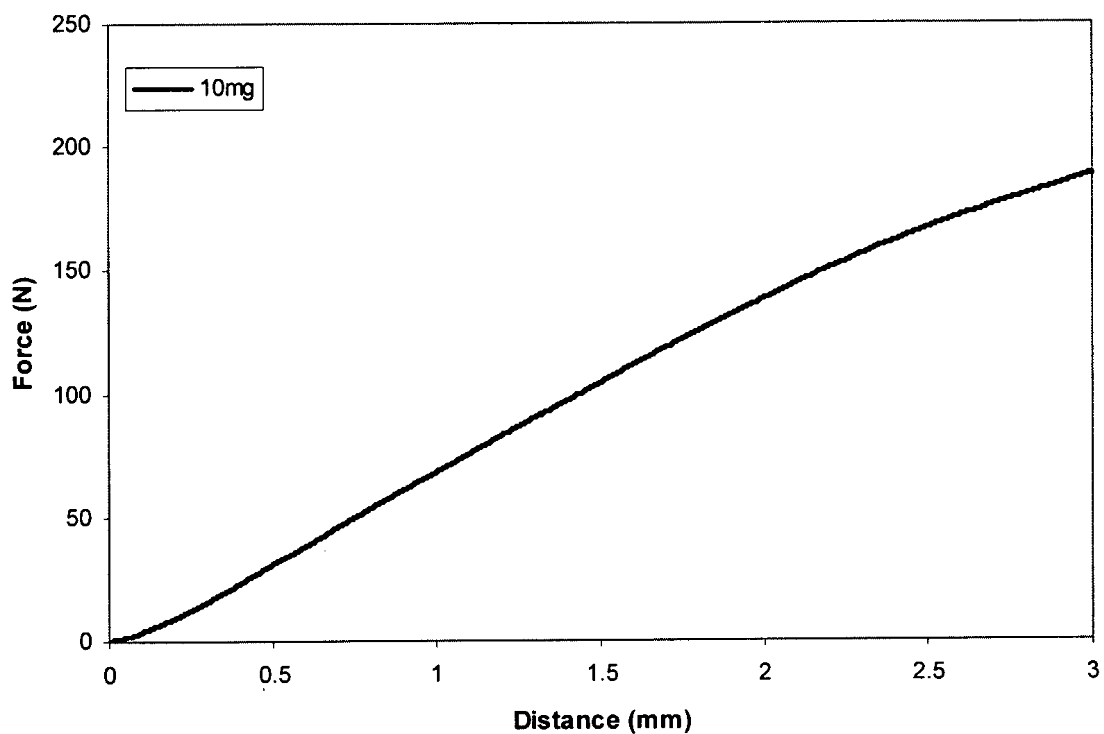
Example 20 Indentation Test of Example 13.1 tablet
