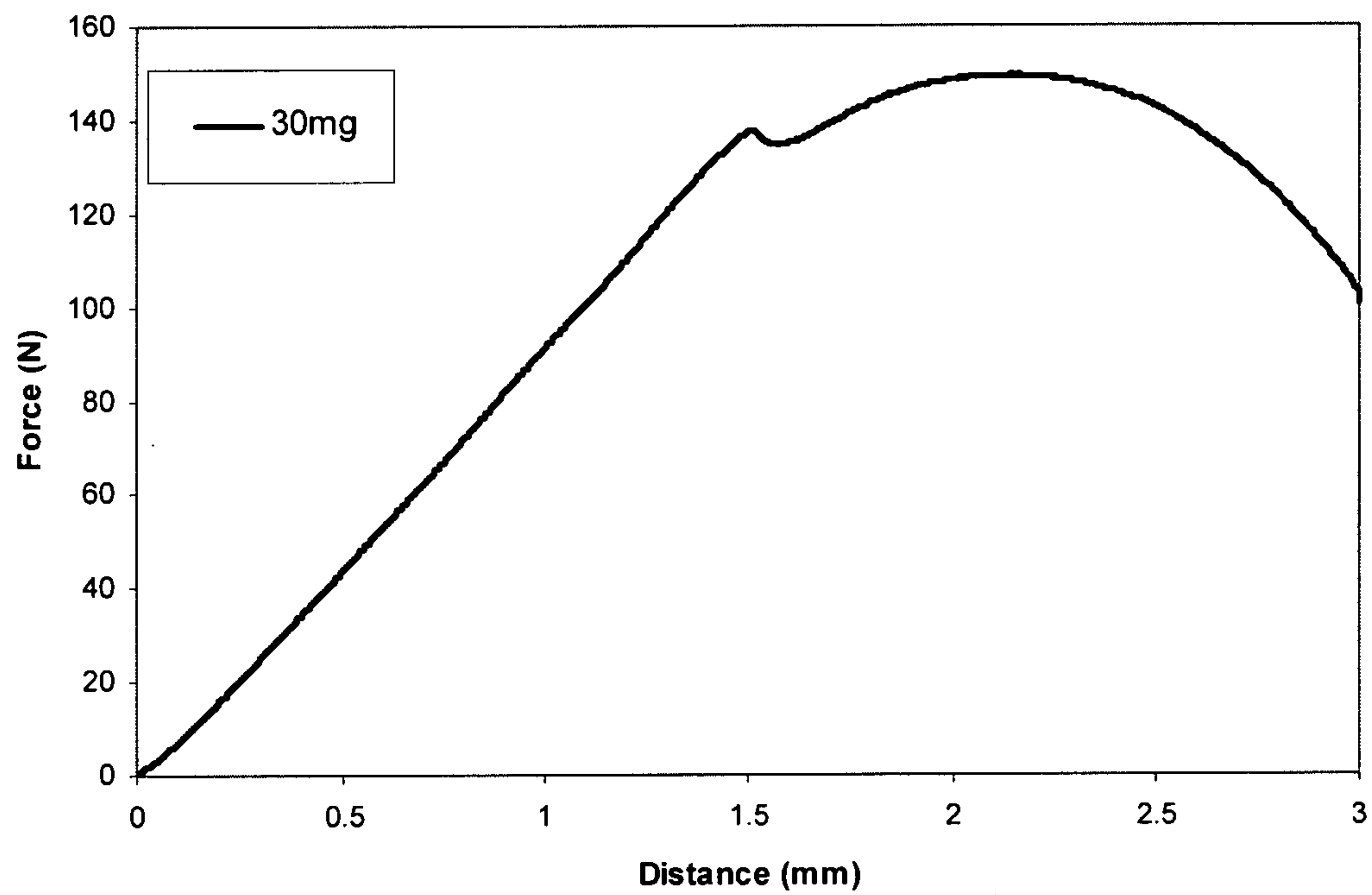
Example 20 Indentation Test of Example 14.4 tablet
