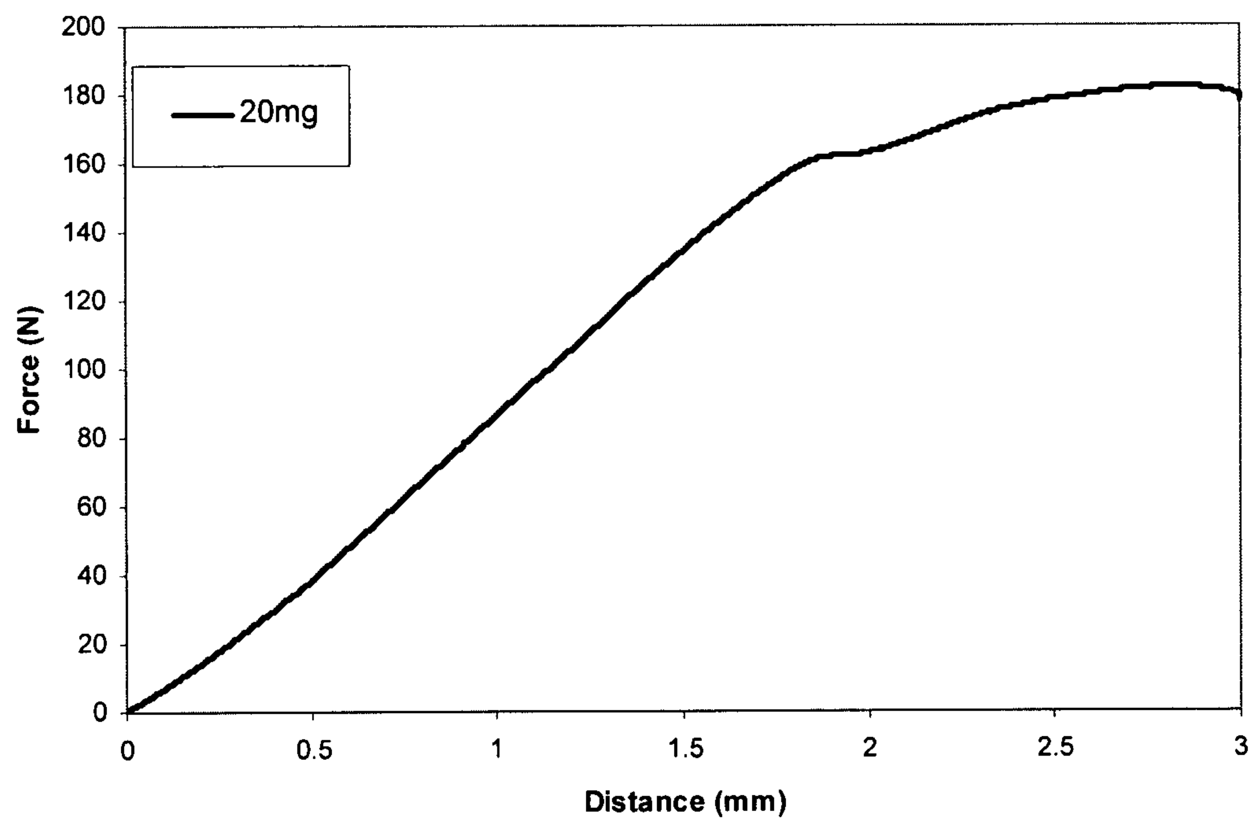
Example 20 Indentation Test of Example 14.3 tablet
