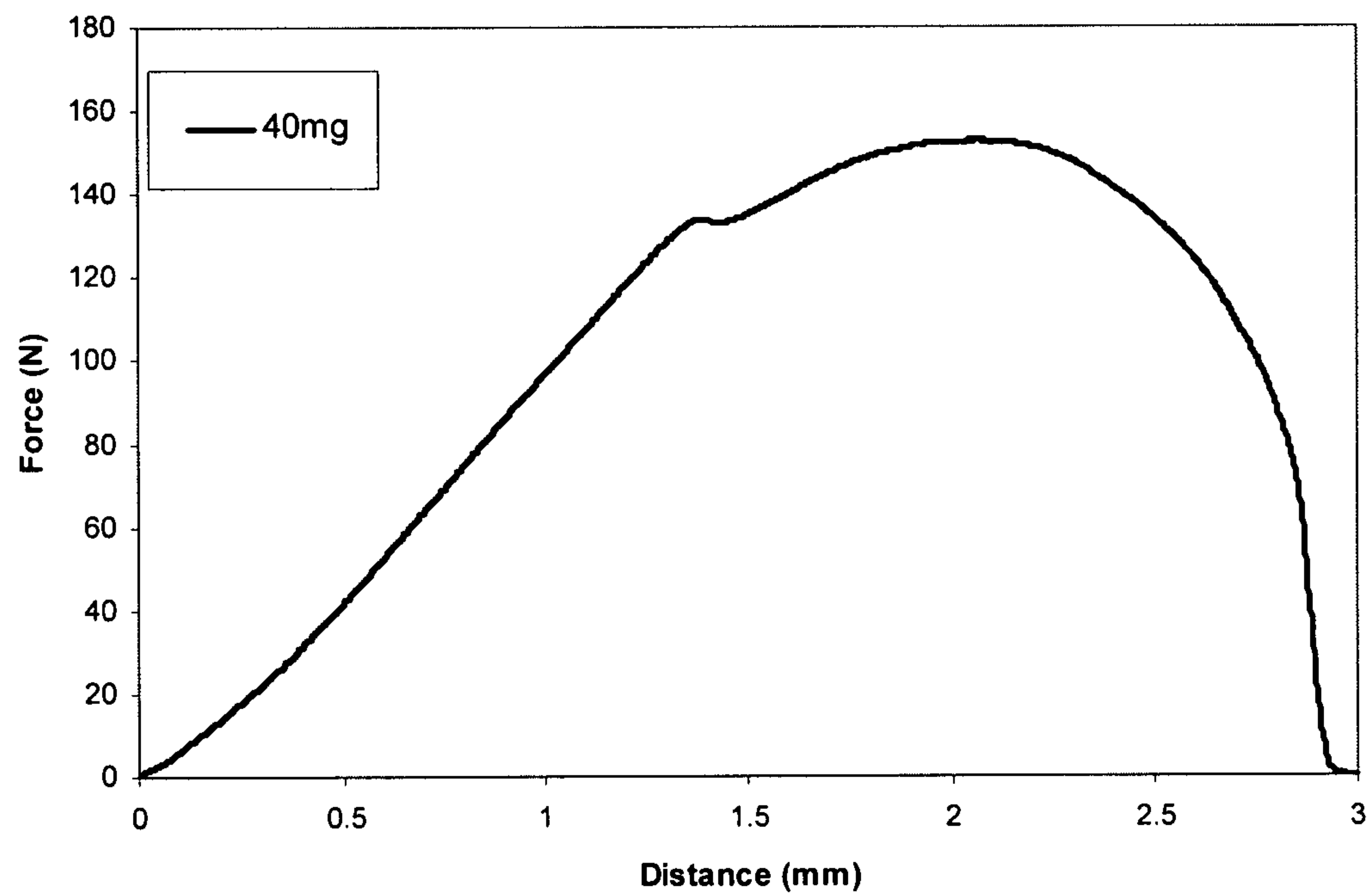
Example 20 Indentation Test of Example 14.5 tablet
