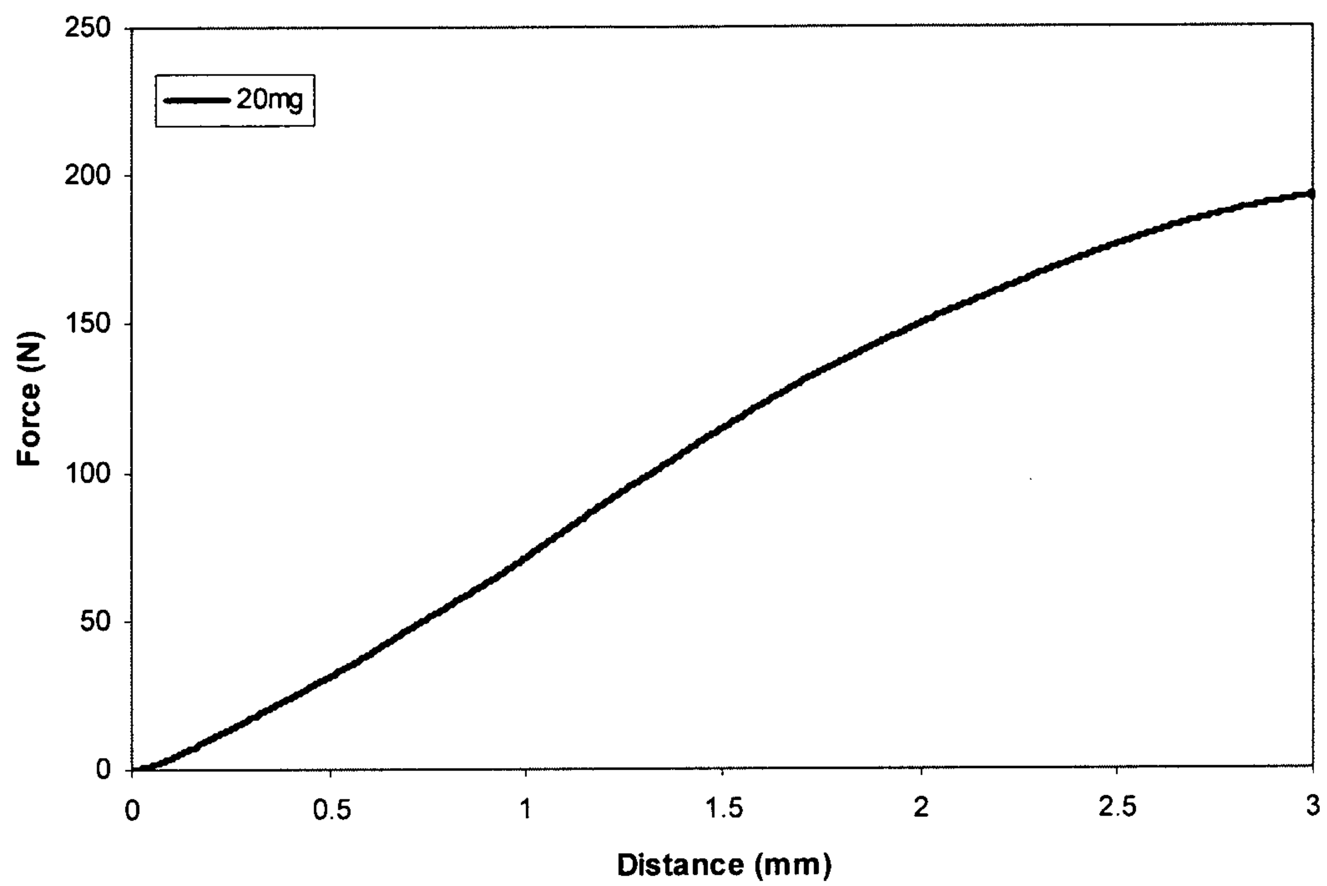
Example 20 Indentation Test of Example 13.3 tablet
