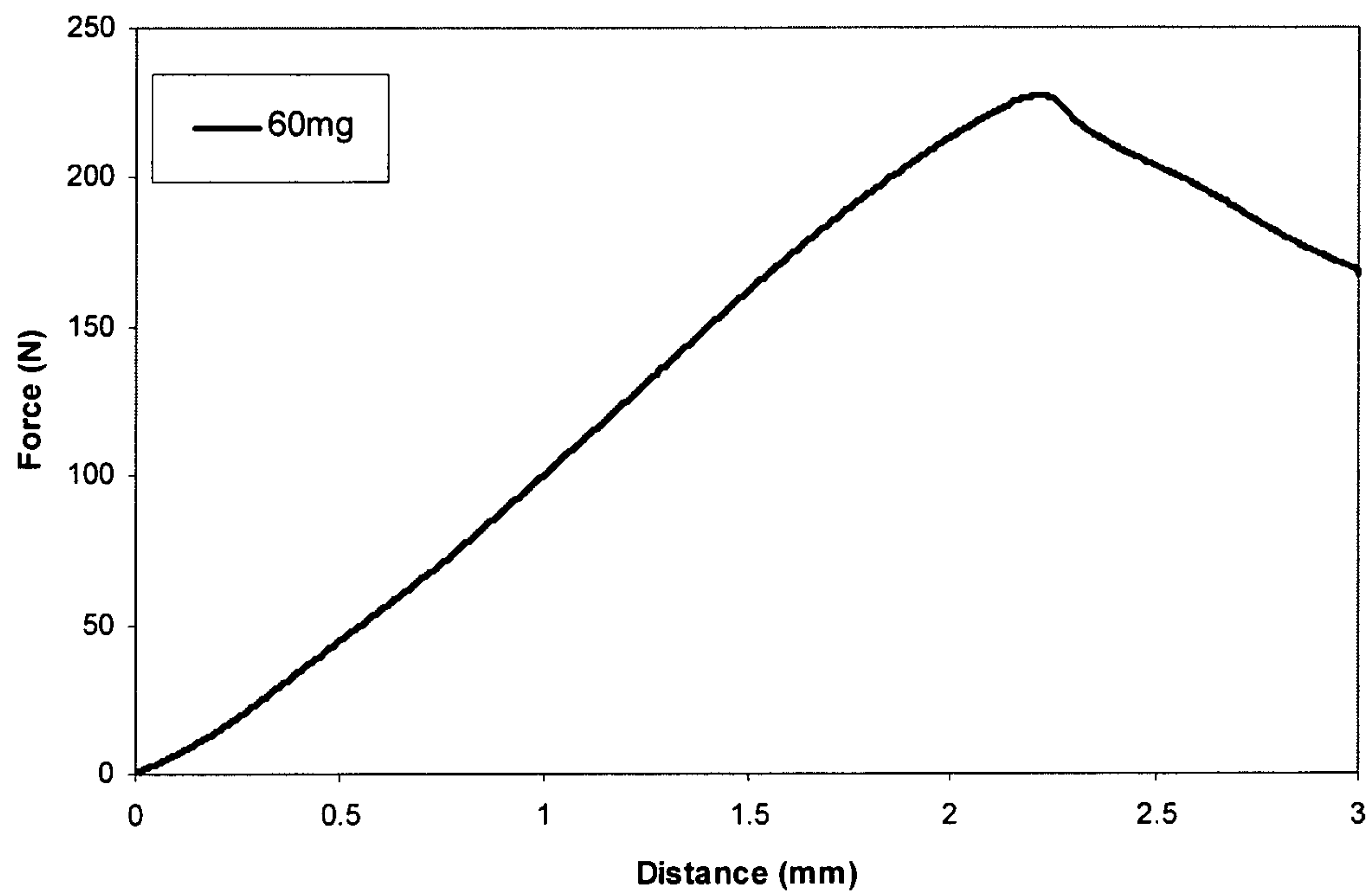
Example 20 Indentation Test of Example 16.1 tablet
