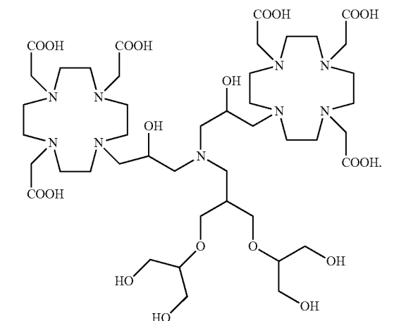
Compound 8
