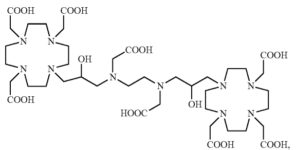
Compound 6
