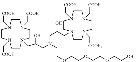
Compound 8
