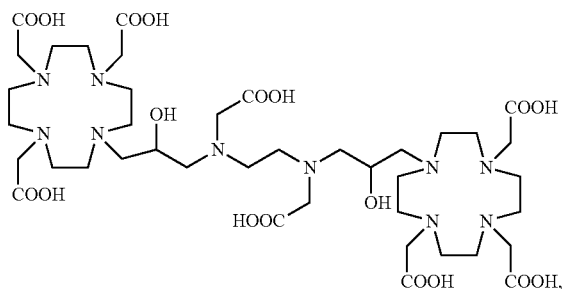
Compound 6
