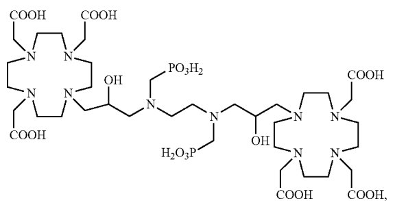
Compound 7
