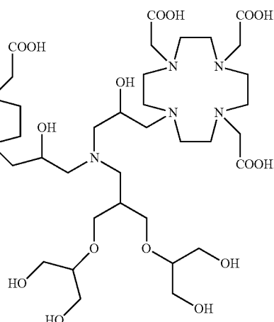
Compound 8
