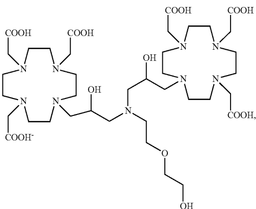
Compound 5
