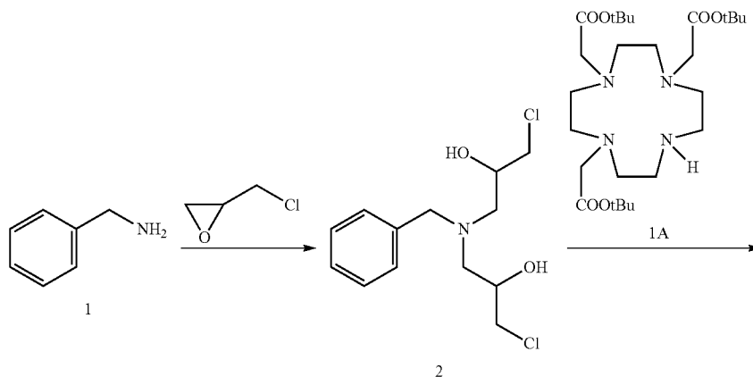
Scheme 7
