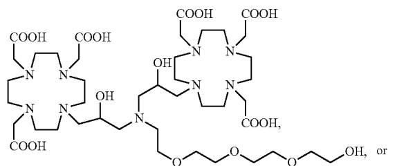
Compound 7
