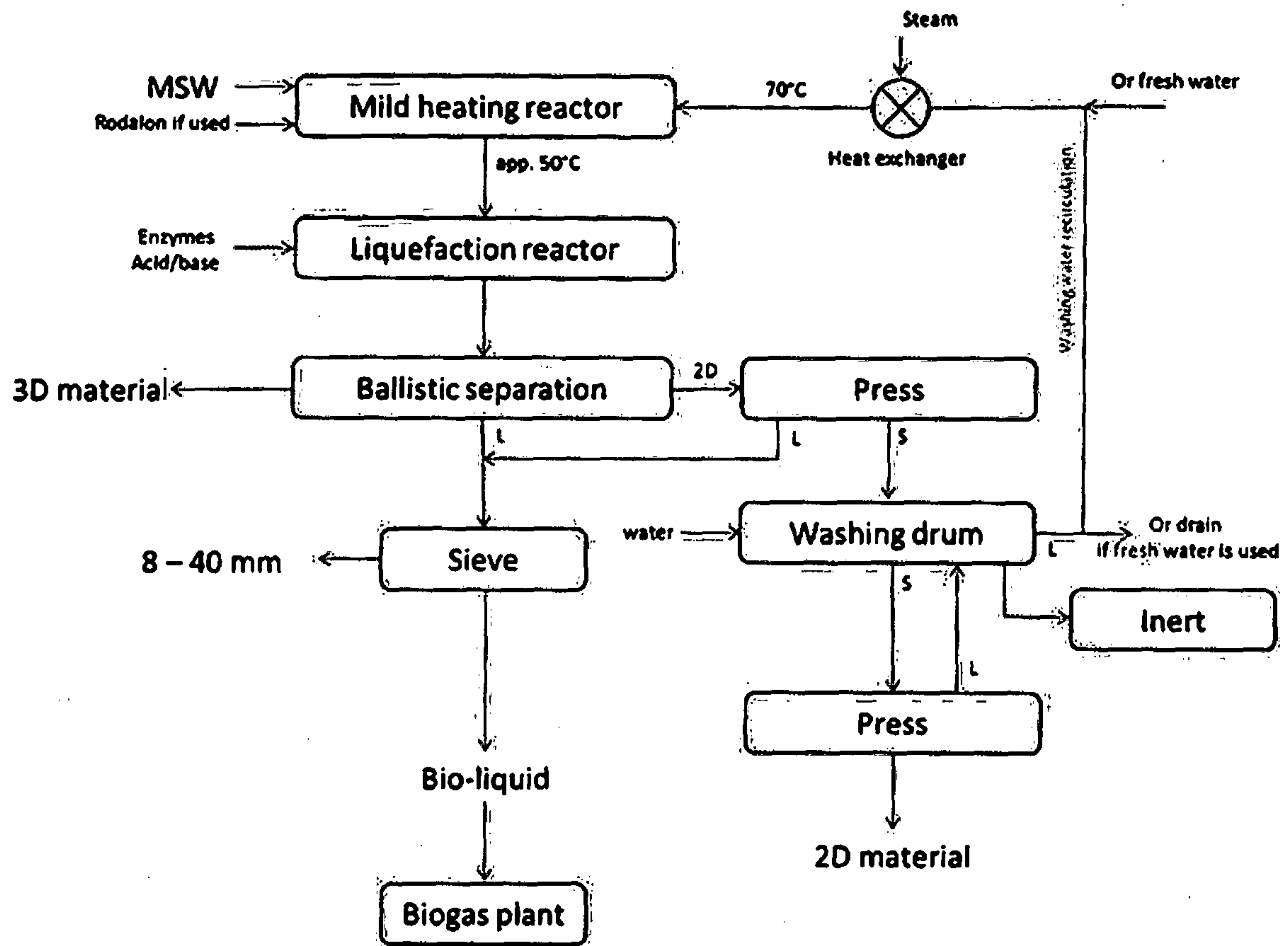
Figure 4. Schematic illustration of demonstration plant set-up.
