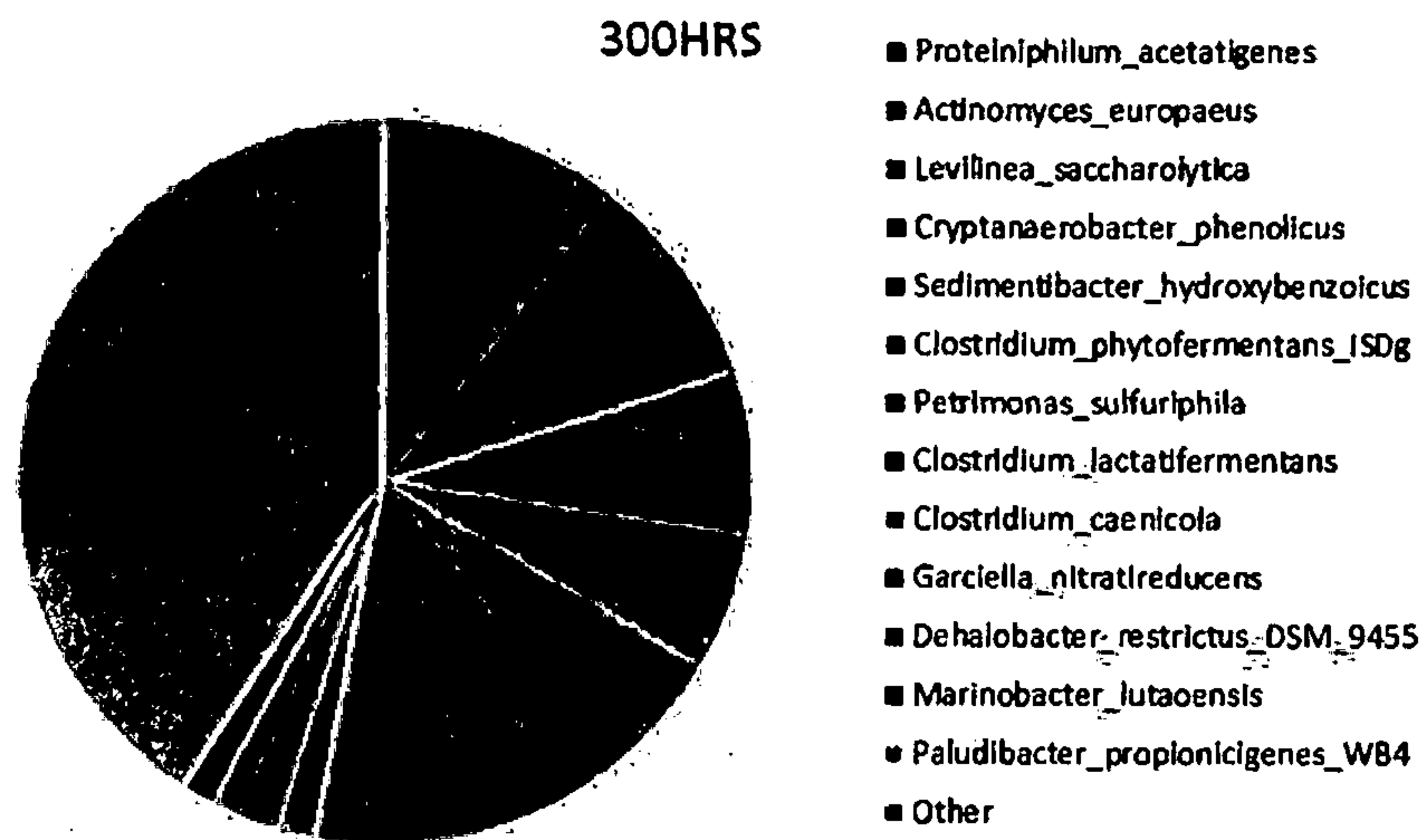
Figure 8 Distribution of the 13 predominant bacteria in the EC12B sampled from the test described in example 5.
