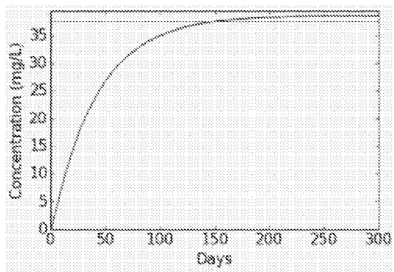
Figure 22b: Simulated Human Plasma Concentration Profile for Alirocumab delivered daily as a 10.5 mg dose using swallowable device embodiments of the invention.
