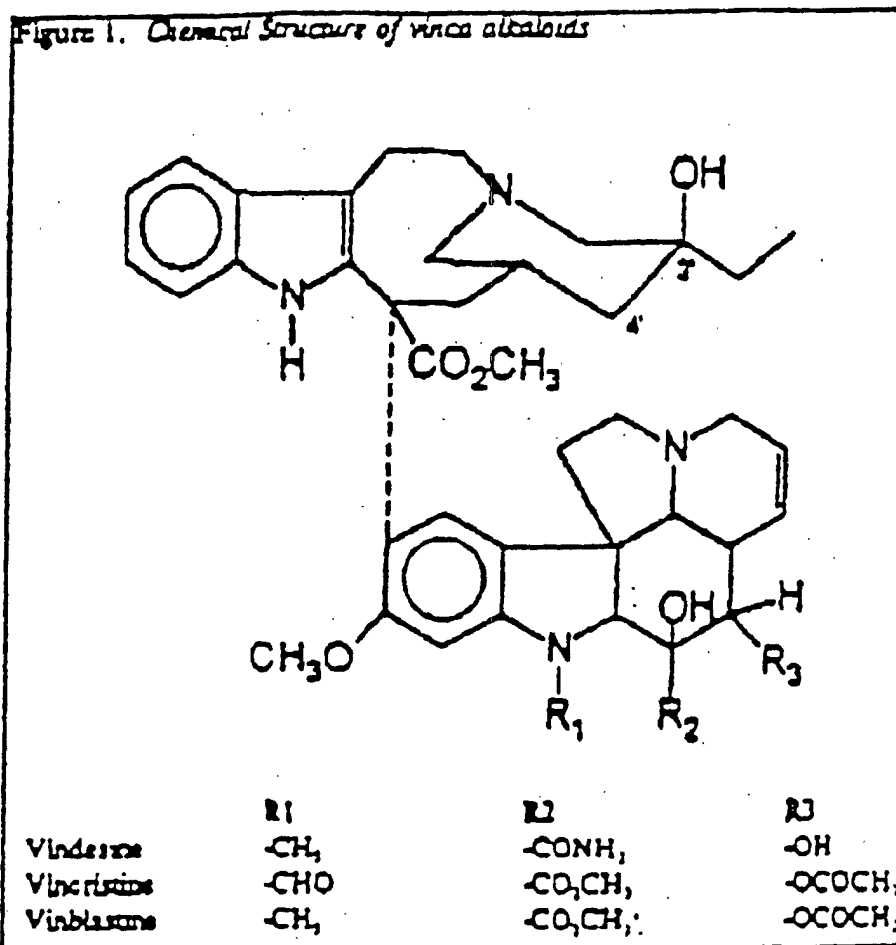
FIGURE 1: Chemical structure of some vinca alkaloids.
