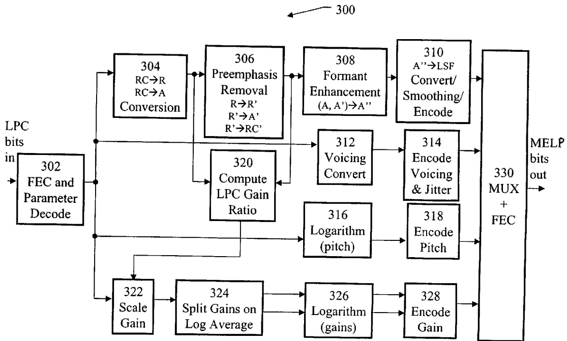
LPC to MELP Transcoder
