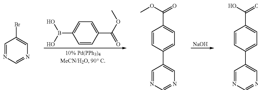
Scheme 23
