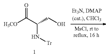
Scheme 42
