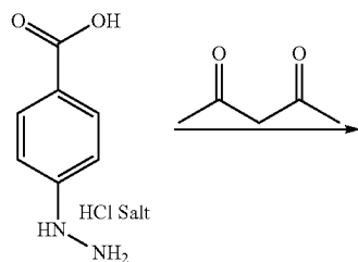
Scheme 30
