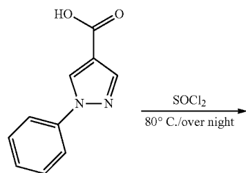
Scheme 38
