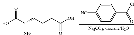
Scheme 27
