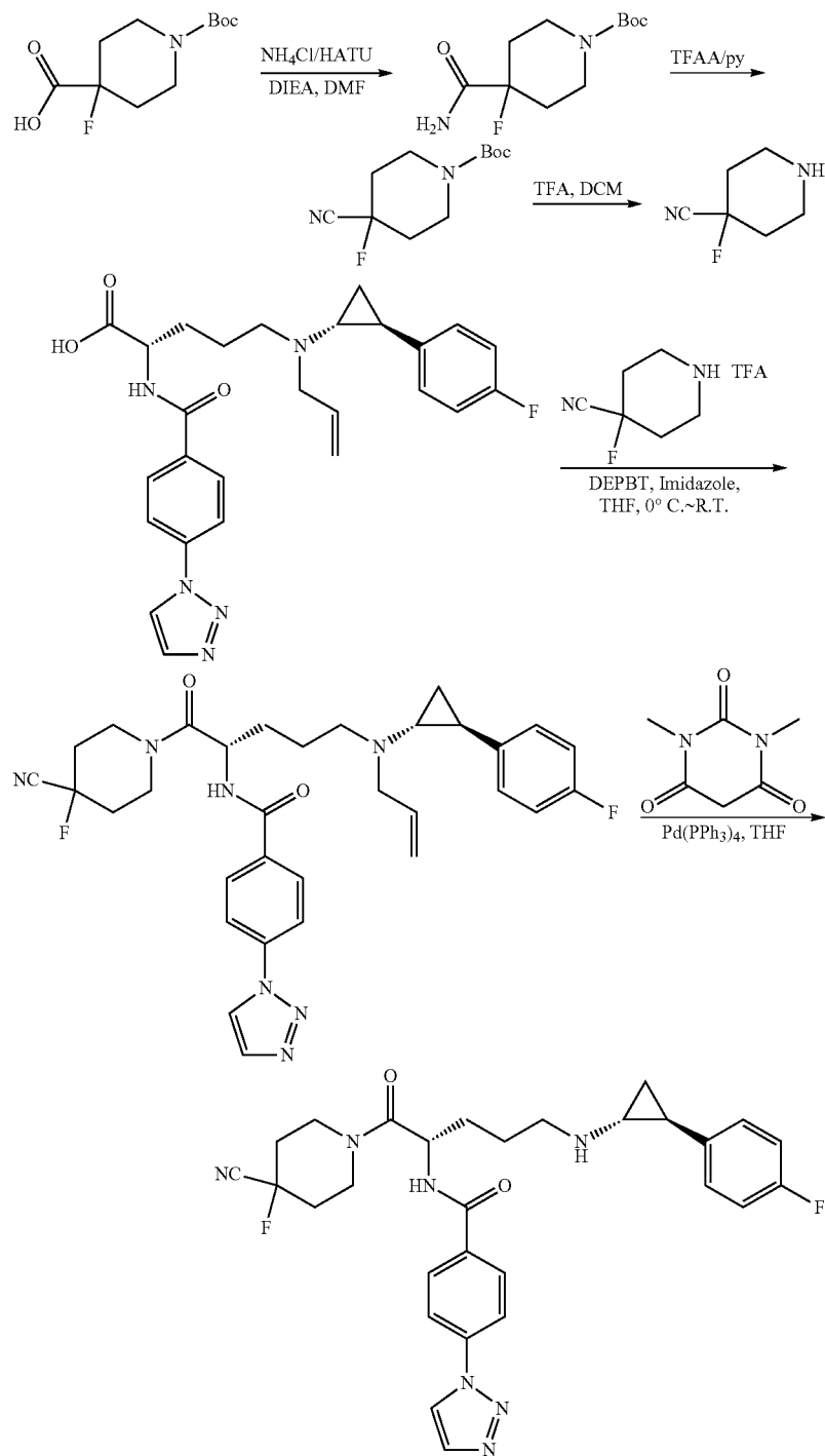
Scheme 20
