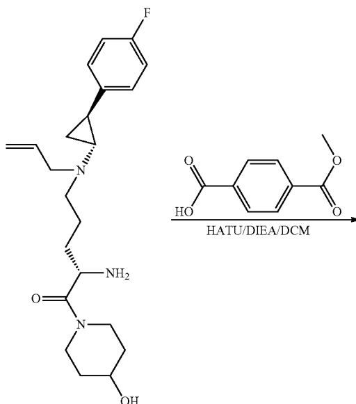
Scheme 11
