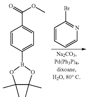
Scheme 35
