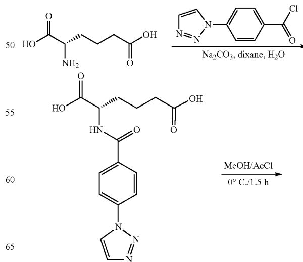
Scheme 26
