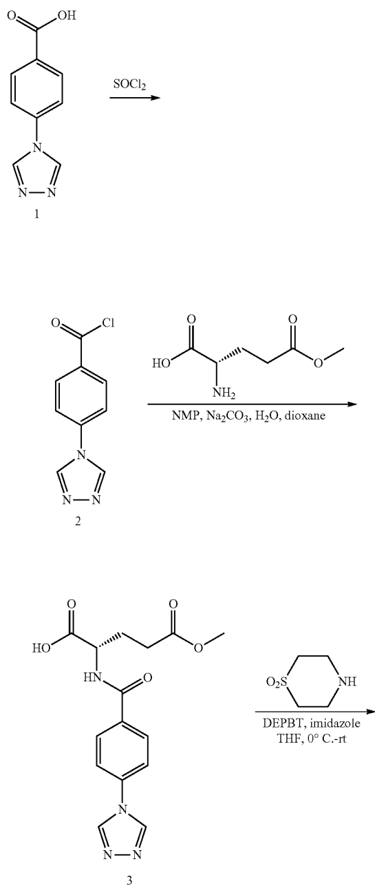
Scheme 36
