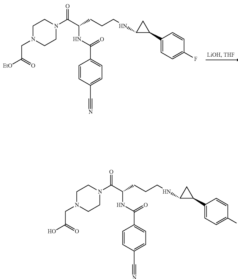
Scheme 15
