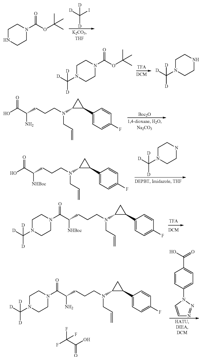
Scheme 24
