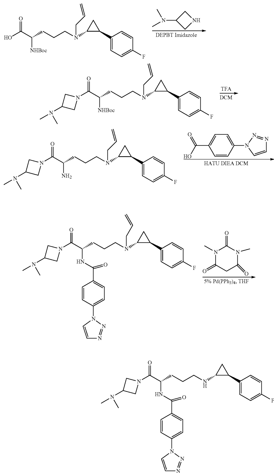
Scheme 14
