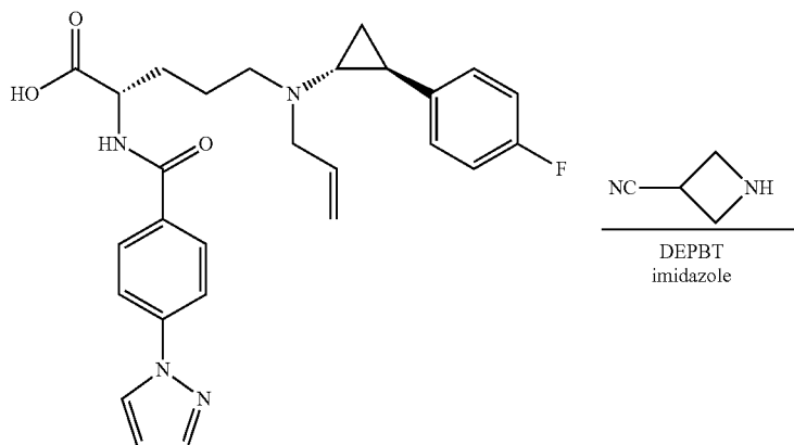
Scheme 7
