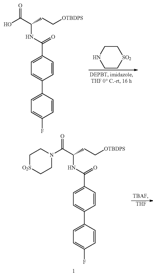
Scheme 44
