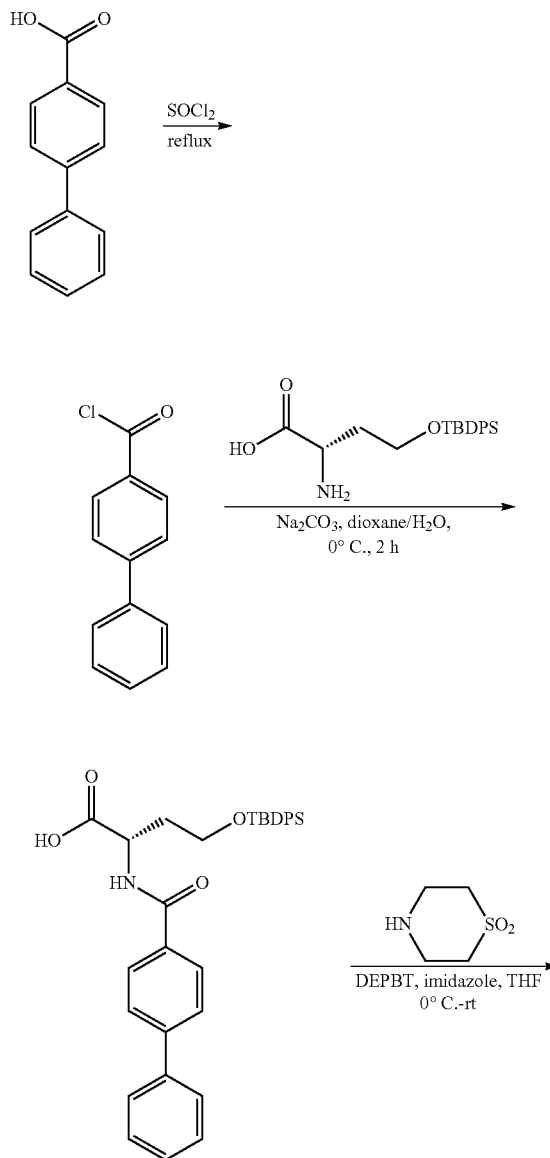
Scheme 2
