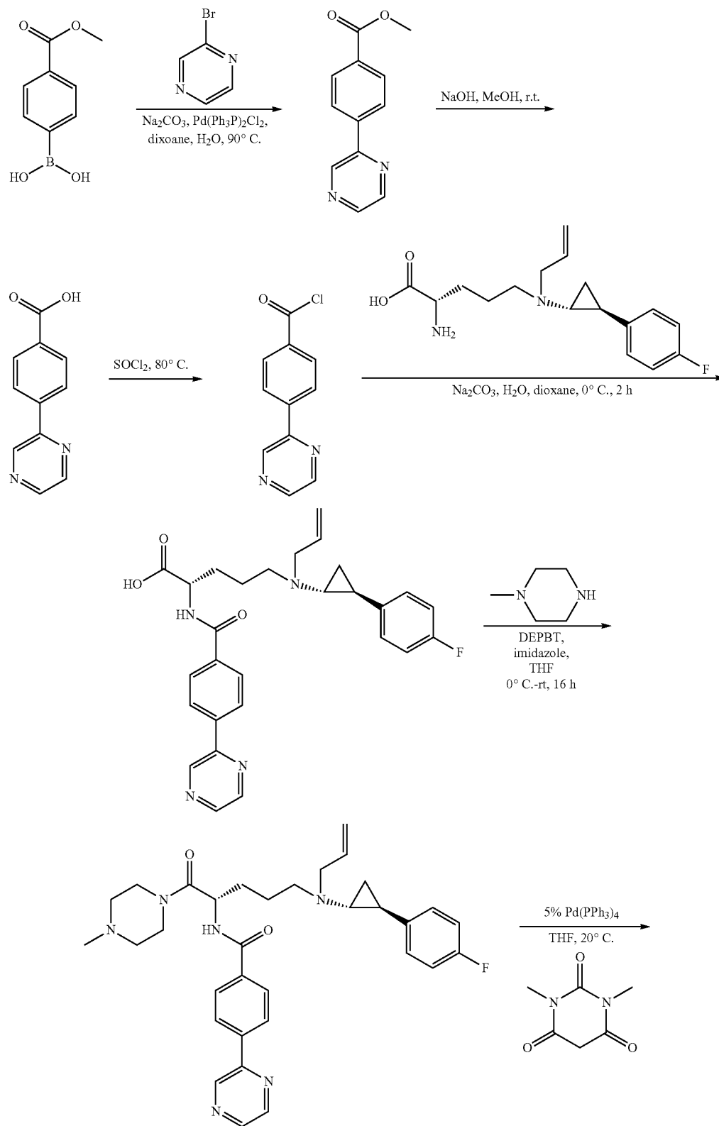
Scheme 22
