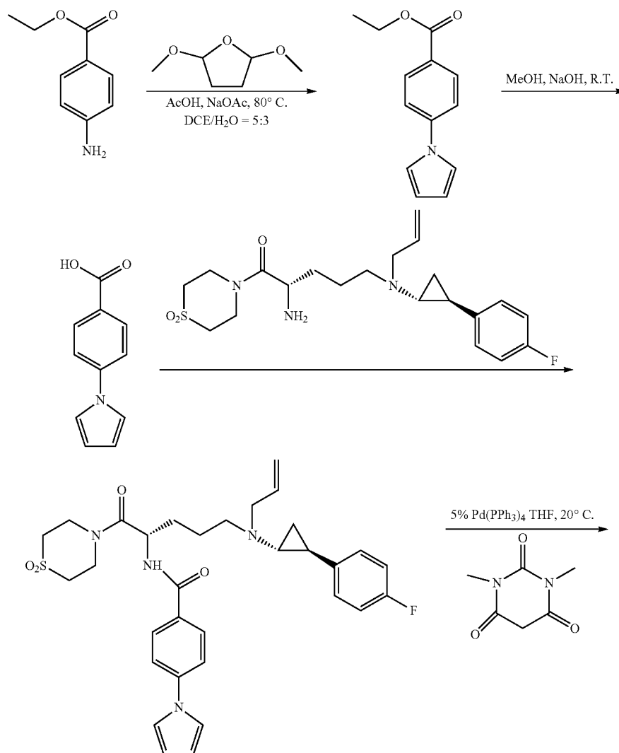
Scheme 40
