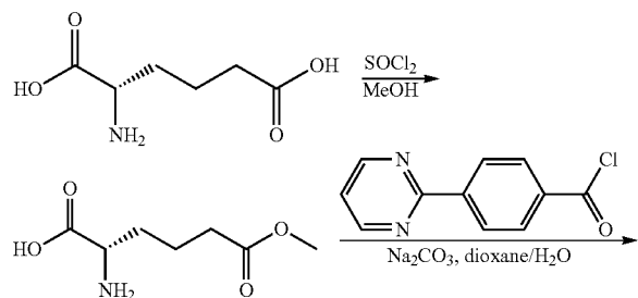
Scheme 28
