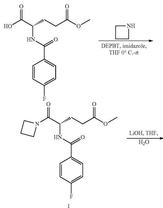
Scheme 45
