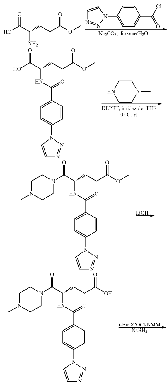
Scheme 18
