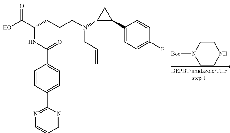
Scheme 8
