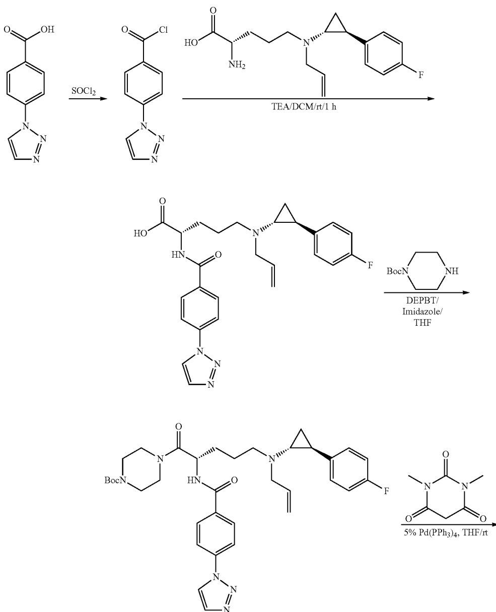
Scheme 6
