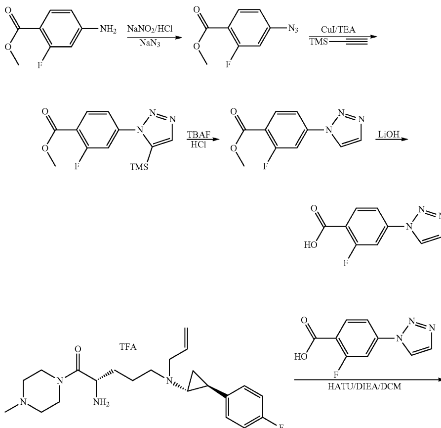
Scheme 19
