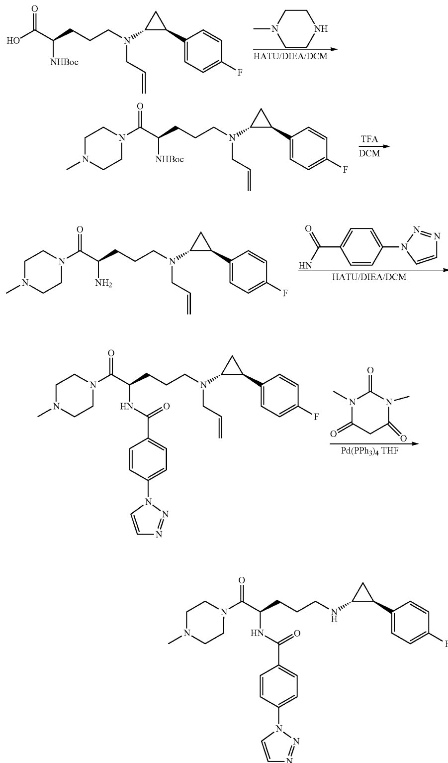
Scheme 12
