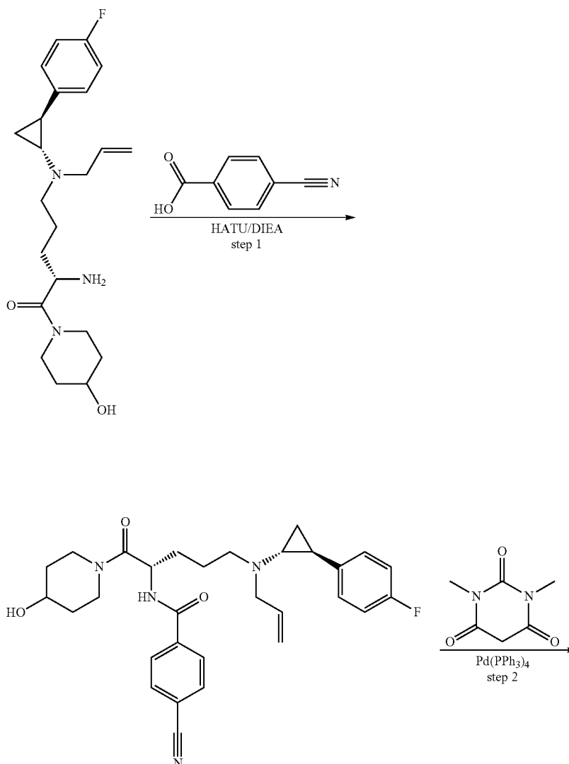
Scheme 10
