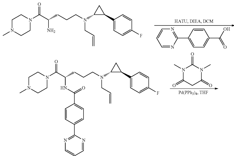
Scheme 41
