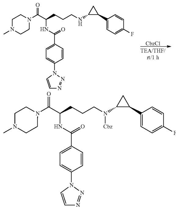
Scheme 16
