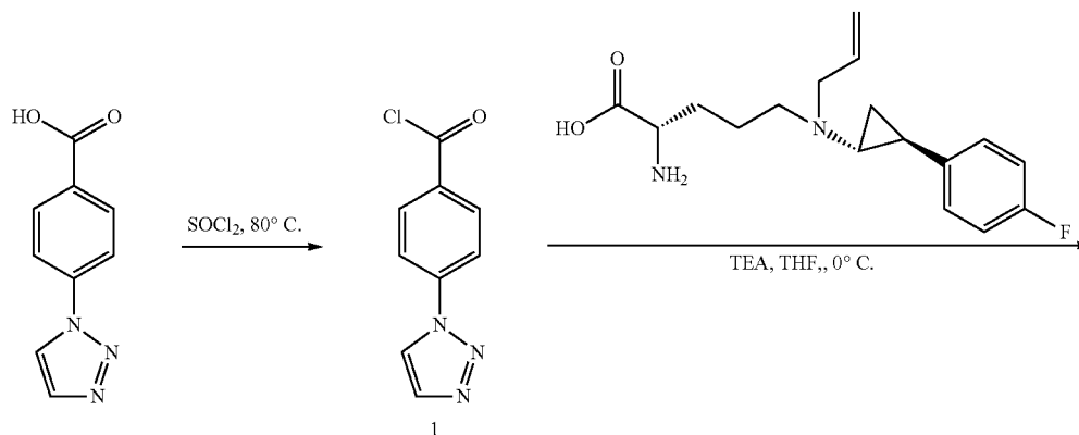
Scheme 34 (a)
