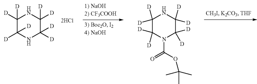
Scheme 25
