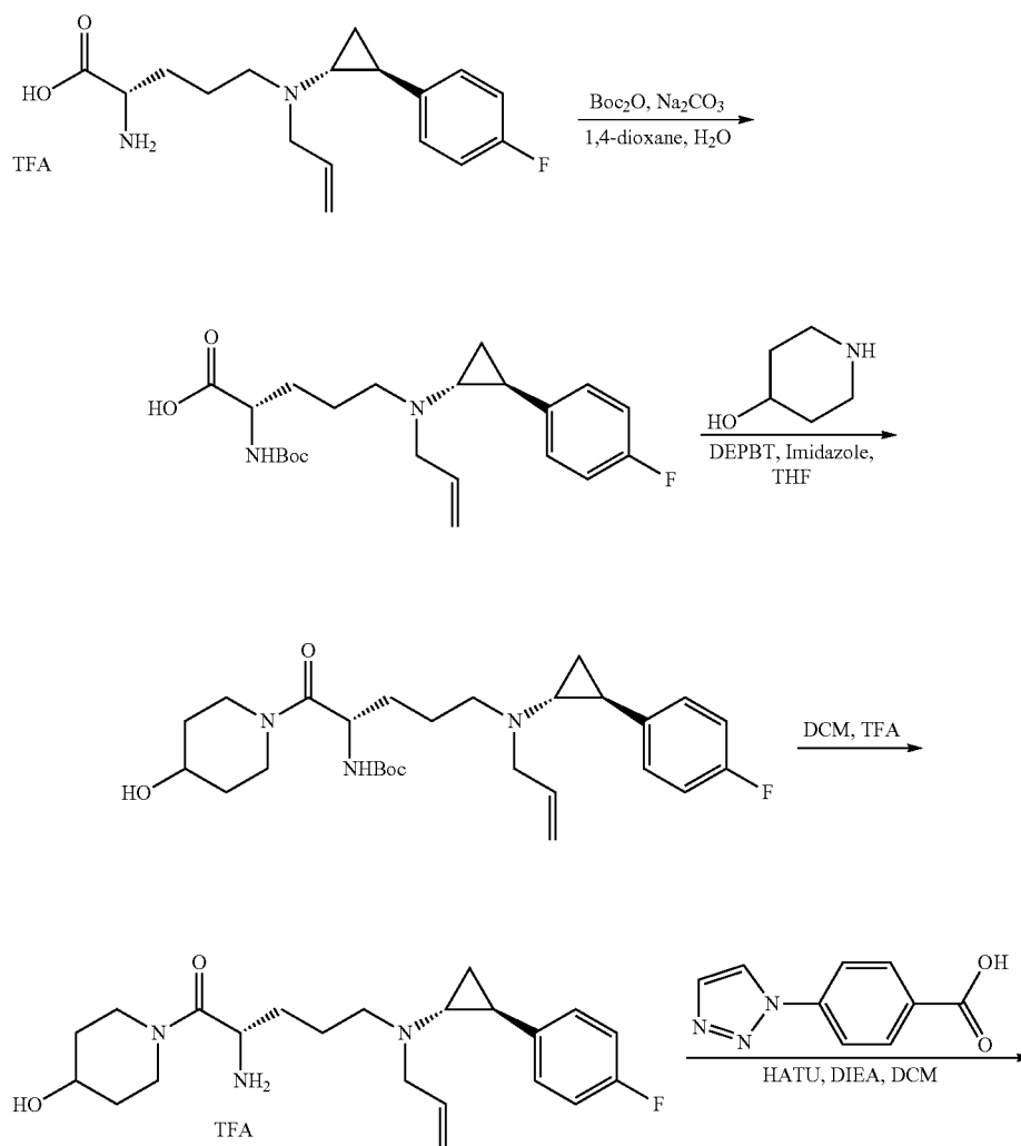
Scheme 13
