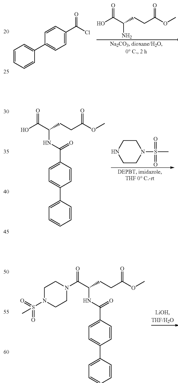
Scheme 17
