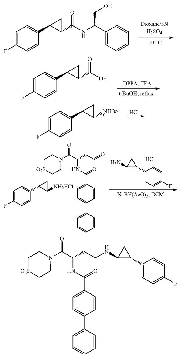
Scheme 32
